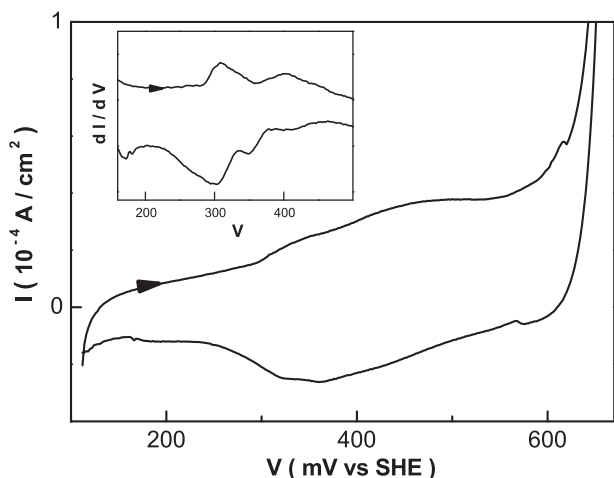
Fig. 3. Splitting of the \text{Ir}^{5+/4+} couple peaks observed at low sweep speed ( 5 \cdot 10^{-4} V/s) on a cleaved (001) \text{Sr}_2\text{IrO}_4 single crystal surface (1 M KOH).
