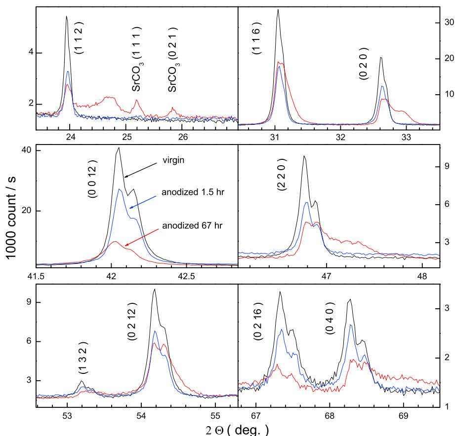
Fig. 6. X-ray diffraction spectra, prior and after anodizing a sintered \text{Sr}_2\text{IrO}_4 sample at 510 mV in 1 M KOH for 1.5 h (blue curve) and 67 h (red curve). (For interpretation of the references to colour in this figure legend, the reader is referred to the web version of this article.)
