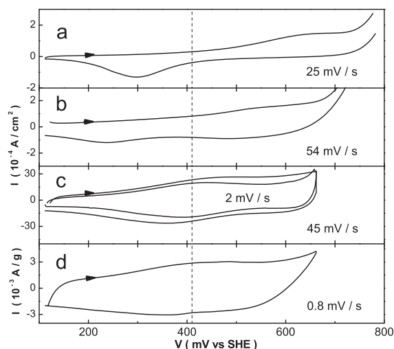
Fig. 4. Cyclic voltammograms for different \text{Sr}_2\text{IrO}_4 samples (1 M KOH). a: cleaved single crystal, b: thin film, c: abraded single crystal, d: sintered powder. The dotted line at 410 mV is the estimated \text{Ir}^{5+/4+} redox potential.
