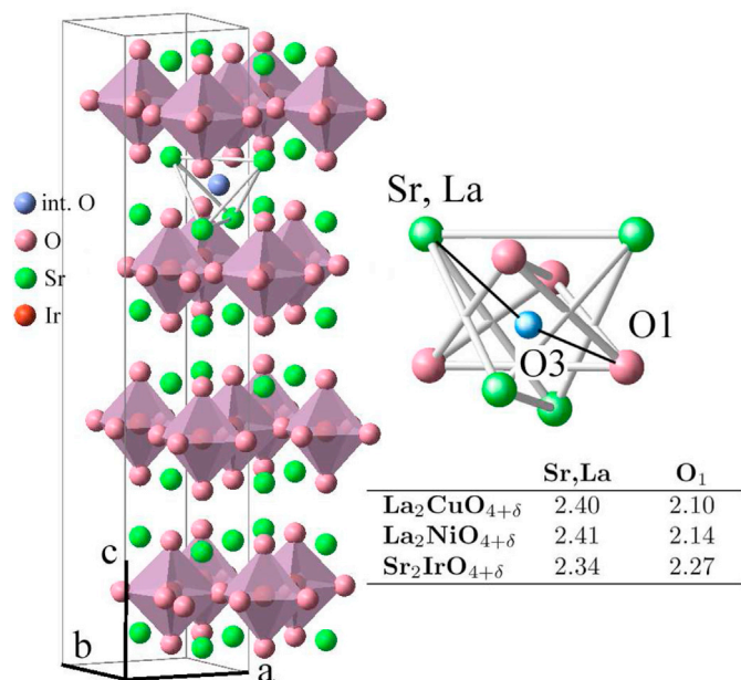
Fig. 1. Representation of the interstitial oxygen atom in \text{Sr}_2\text{IrO}_{4+\delta} , assuming it is similar to the one in \text{La}_2\text{CuO}_{4+\delta} and \text{La}_2\text{NiO}_{4+\delta} . The atomic distances in table are the ones for the undistorted structure to \text{O}_3 ( \frac{1}{2}\text{O}_3^2 ) (averaged, in the case of \text{La}_2\text{CuO}_4 and \text{La}_2\text{NiO}_4 , for which there is a tilt of the oxygen octahedra).
