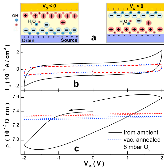
Fig. 10. Gating with ionic liquid the 88 nm thick \text{Sr}_2\text{IrO}_4 film (b: gate current, c: film resistivity. T = 220 \text{ K} ). Full line is for ionic liquid applied in ambient conditions, dotted line is for pumping first on ionic liquid at 300 \text{ K} , 10^{-5} \text{ mbar} for 1 h, both then measured in 10 mbar He thermal exchange gas. Dashed line is for pumped ionic liquid cooled down to 220 \text{ K} in 8 mbar \text{O}_2 . a: sketch of water dissociation upon gating (after Ref. [41]). dV_G/dt = 2 \text{ mV/s} .
