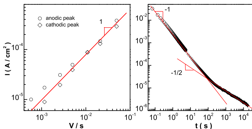
Fig. 7. Left: anodic and cathodic peak current dependence on sweep speed (cleaved (001) \text{Sr}_2\text{IrO}_4 single crystal surface, in 1 M KOH). Right: relaxation of the cathodic current, after application of a step voltage from 460 mV to 110 mV (crosses and circles are obtained from two distinct acquisitions).
