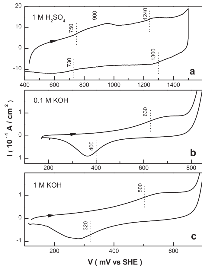
Fig. 2. Cyclic voltammograms for a cleaved (001) \text{Sr}_2\text{IrO}_4 single crystal surfaces (from top to bottom: dV/dt = 50, 10, 14 \text{ mV/s} , \text{pH} = 0.3, 13, 14 ). The dotted lines indicate the steepest slope location of the redox peaks.
