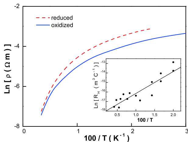
Fig. 8. Resistivity of an 88 nm-thick film, after reduction (110 mV) and oxidation (460 mV) in 1 M KOH. The inset shows the Hall number, for the reduced film. The line is a fit to an Arrhenius law, with activation energy 20 meV.
