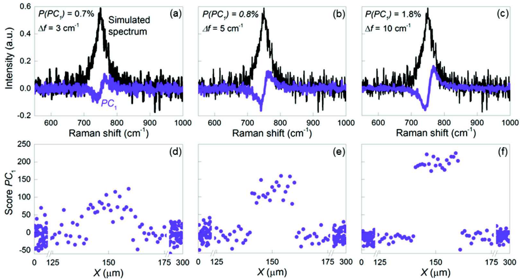
Figure 3. Influence of the amplitude of the frequency shift on noisy spectra. PC obtained when performing PCA on spectra with a SNR of 10 and a frequency shift of (a) 3 \text{ cm}^{-1} , (b) 5 \text{ cm}^{-1} and (c) 10 \text{ cm}^{-1} . (d)–(f) are the corresponding scores for every spectrum.
