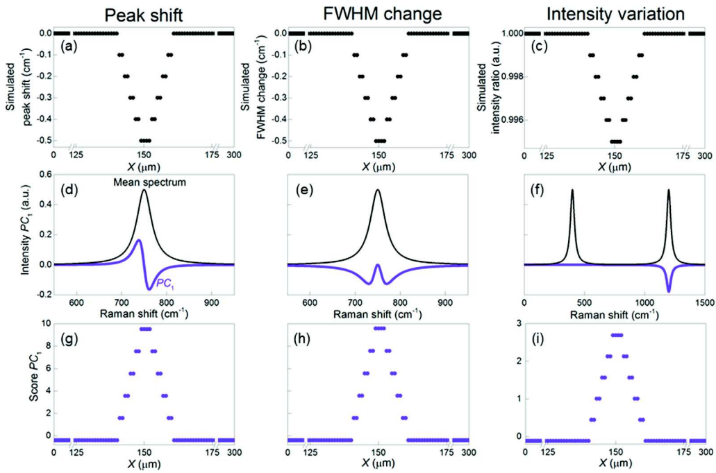
Figure 1. PCA results for simulated hypothetical spectra. Three hypothetical domain wall signatures are applied to 20 Lorentzian: (a) a shift of a single peak, (b) a change in the FWHM of a single peak and (c) an intensity variation between two peaks. The resulting signature of the principal component and mean spectrum are displayed in parts (d)–(f), while parts (g)–(i) present the corresponding scores.
