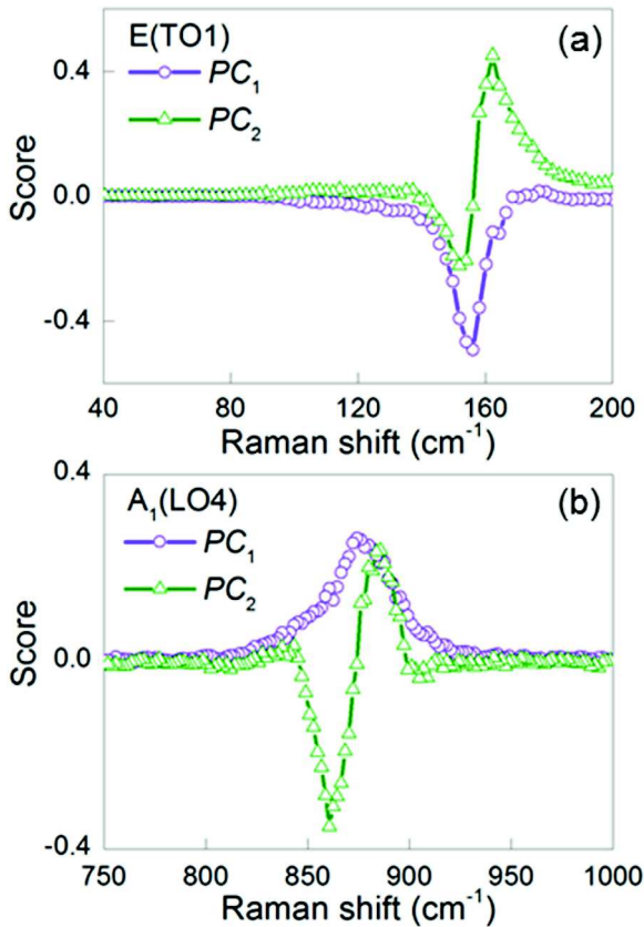
Figure 6. Results of the PCA analysis on individual modes. Scores of the first and second components for (a) E(\text{TO1}) and (b) A_1(\text{LO4}) .
