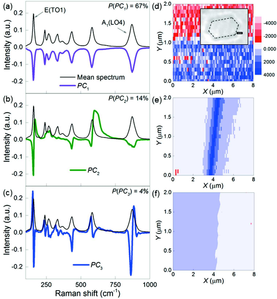
Figure 5. PCA Raman maps of ferroelectric domains and domain walls in LiNbO 3 . Mean spectrum and (a) first PC, (b) second PC, (c) third PC. (d)–(f) are the corresponding scores for every spectrum. The inset in (d) is an optical image of the domain with the investigated area indicated by the black rectangle and the DWs by dashed lines below them.
