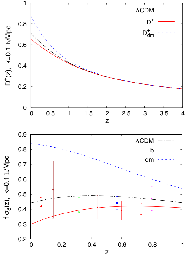
FIG. 9. Upper panel: linear growing modes D^+(k, a) and D_{\text{dm}}^+(k, a) , for the symmetric model of Fig. 1, at comoving wave number k = 0.1 h/\text{Mpc} . Lower panel: growth factors f \sigma_8 and f_{\text{dm}} \sigma_{\text{dm}8} .
