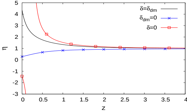
FIG. 11: Gravitational slip \eta of Eq.(87) for several values of the baryon to dark matter ratio \delta/\delta_{dm} .
