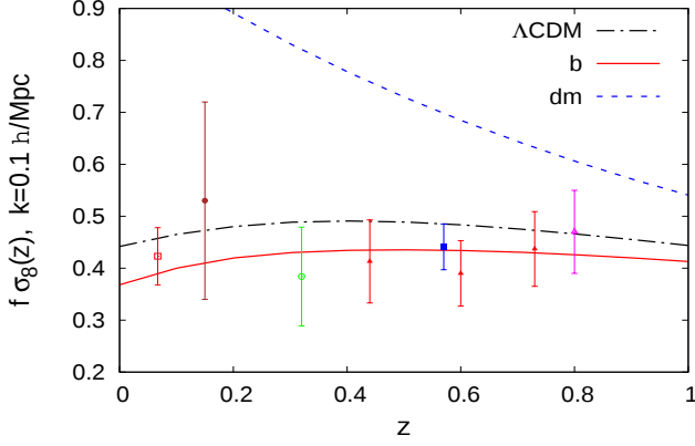
FIG. 10: Growth factors f\sigma_8 and f_{dm}\sigma_{dm8} , for the model of Fig. 4 with different conformal times.
