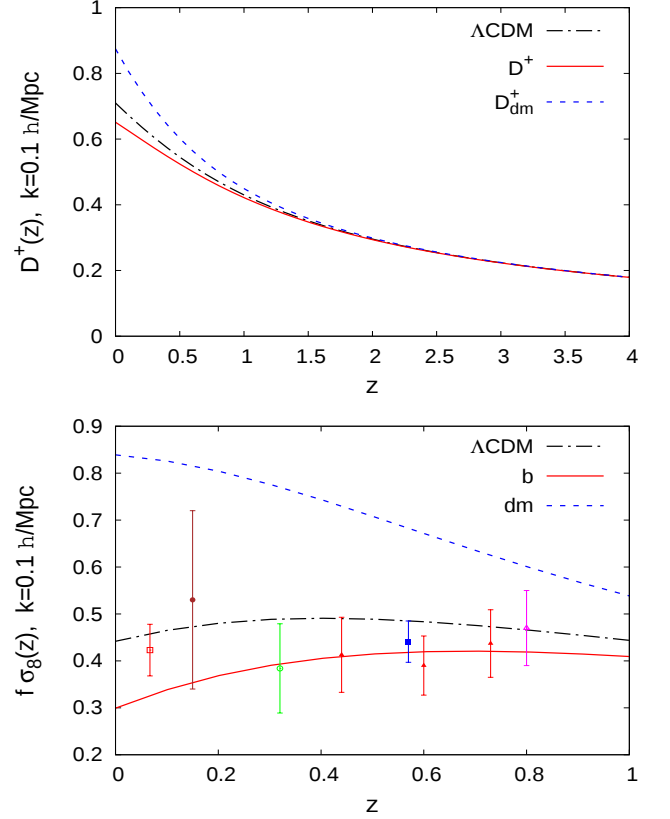
FIG. 9: Upper panel: linear growing modes D^+(k, a) and D_{\text{dm}}^+(k, a) , for the symmetric model of Fig. 1, at comoving wave number k = 0.1 h/\text{Mpc} . Lower panel: growth factors f \sigma_g and f_{\text{dm}} \sigma_{\text{dm}8} .
