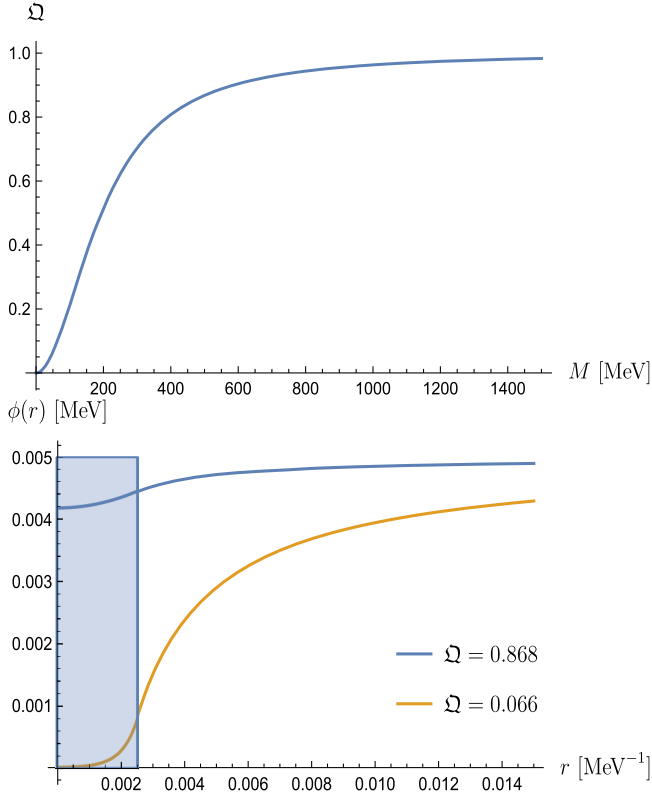
FIG. 3. Top: Here the screening charge \Xi is plotted as a function of the coupling parameter M . The parameters taken are for a neutron, viz. R = 2.5 \times 10^{-3} \text{ MeV}^{-1} , \rho_n = 1.53 \times 10^{10} \text{ MeV}^4 and \mu = 5 \times 10^{-8} \text{ MeV} . Bottom: The field profile of a sphere (neutron) is plotted as a function of the radial distance of the center of the sphere. The blue line corresponds to M = 500 \text{ MeV} and the yellow line to M = 50 \text{ MeV} with the other parameters having the same values as those used for the upper plot. The blue square is bounded by the radius of the sphere (neutron) and the vacuum field value \phi = \phi_v .
