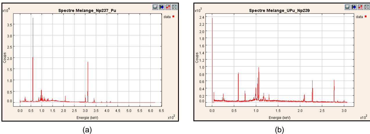
Figure 3 – Spectra (a) of plutonium with a substantial amount of ^{237}\text{Np}/^{233}\text{Pa} and (b) of a mixture of uranium and plutonium with a substantial amount of ^{243}\text{Am}/^{239}\text{Np}
