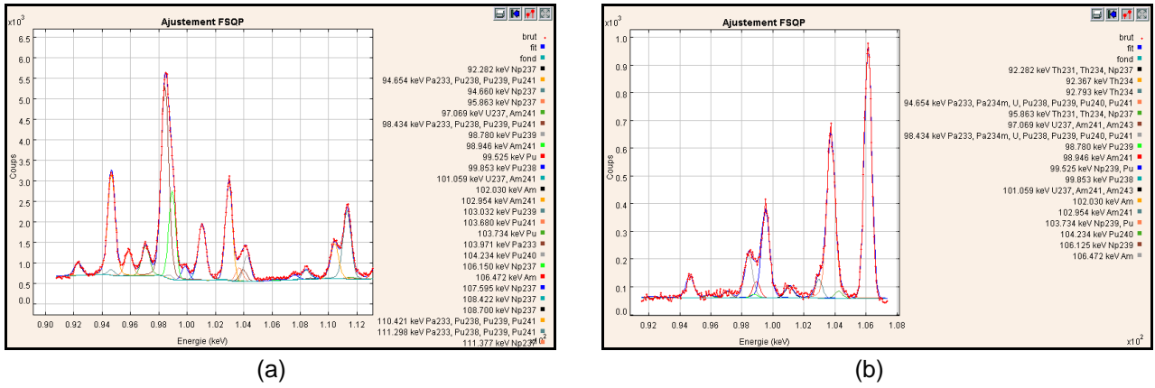
Figure 4 – Examples of deconvolution of a complex region by the region analysis module, for spectra (a) with \text{Pu}^{237}\text{Np}/^{233}\text{Pa} and (b) with \text{UPu}^{243}\text{Am}/^{239}\text{Np}
