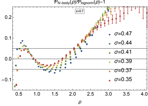
Figure D1. The residuals of the best fit log normal PDF \mathcal{P}(\rho) for redshift z = 0.7 and radii R = 10, 11, \dots, 15 \text{ Mpc/h} (from blue to red) in comparison to the measurement from HR4 (with error bars). This is to be contrasted to the quasi perfect match of the saddle PDF presented in Figure 3
