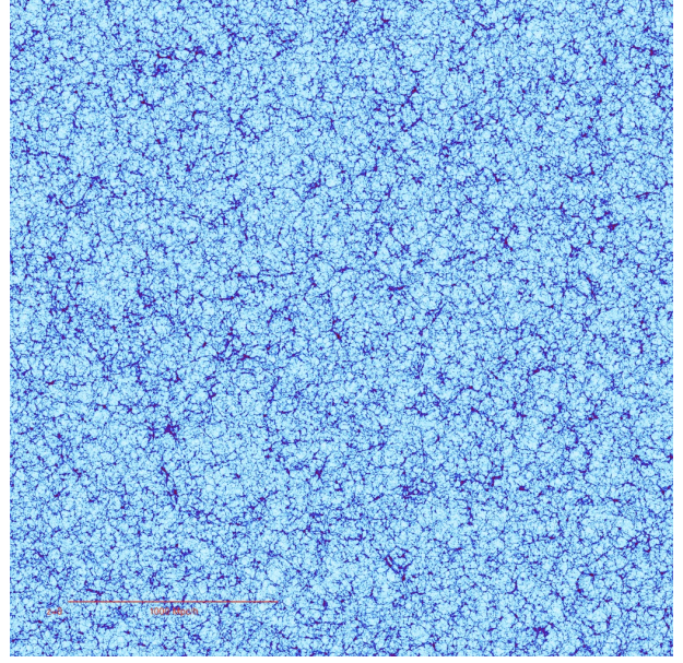
Figure 2. A thin (1.5 Mpc/h) slice through the HR4 simulation at redshift 0. The simulation is 3150 Mpc/h across sampled by 6300 3 dark matter particles.
