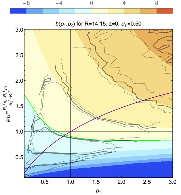
Figure D6. A contour plot of the joint density and slope bias function b(\rho, s) predicted from the saddle point approximation equation (29) with normalization from equation (18) for R_1 = 14 Mpc/h and R_2 = 15 Mpc/h at redshift z = 0 where \sigma_\mu = 0.50 , (corresponding to \sigma_\rho = 0.55 ), in comparison to the measurements from HR4 (mean as thick black lines, and mean \pm error on the mean as thin black lines).
