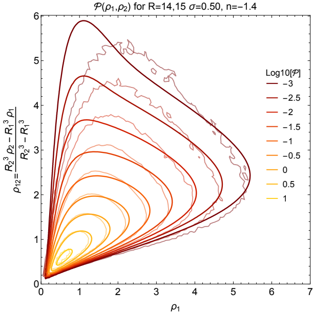
Figure D4. The joint density-slope PDF \mathcal{P}(\rho_1, \rho_2) predicted from equation (25) for radii R_{1,2} = 14, 15 Mpc/h at redshift z = 0 with \nu = 21/13 in comparison to the measurement from HR4 (thin wiggly lines).
