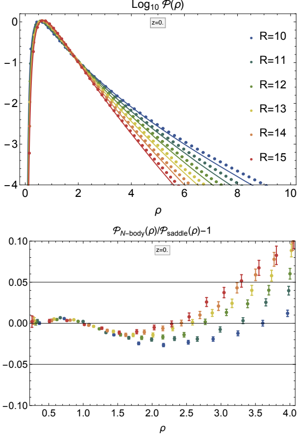
Figure D3. The density PDF \mathcal{P}(\rho) predicted from equation (23) using LSSFast (solid lines) for radii R = 10, 11, \dots, 15 Mpc/h (from blue to red) at redshift z = 0 with a slightly adjusted \nu = 1.59 in comparison to the HR4 measurement (data points) and the corresponding residuals.
