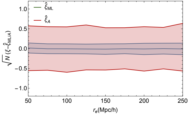
Figure 12. Estimate of the dark matter correlation function at z = 0.7 in 216 random subsamples of N = 222,264 pairs of spheres of radius R = 15 \text{ Mpc}/h separated by r_e = 50 \dots 250 \text{ Mpc}/h . The mean and one standard deviation area are shown in blue for the maximum likelihood estimator \hat{\xi}_{\text{ML}} and in red for the usual sample estimator \hat{\xi}_A . We display only the difference compared to the dark matter correlation function measured in the full simulation which is assumed to be the true underlying value of \xi . As expected, the maximum likelihood estimator provides a much smaller scatter than the sample estimator.
