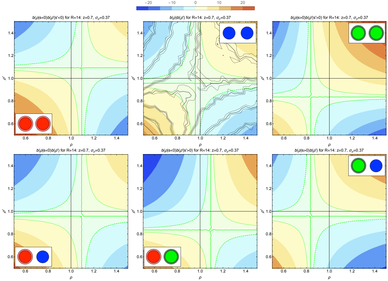
Figure 10. The bias modulation of the two-point sphere correlation function b(\rho)b(\rho') = \xi_o(\rho, \rho'; r_e)/\xi(r_e) for radii R = R' = 14\text{Mpc}/h at redshift z = 0.7 with the variance \sigma_\mu=0.37 computed from the bias and constrained bias in an over- or underdense mass shell shown in Figure 8. Besides equi-bias contours we show the line of zero bias b = 0 (green line) and unity bias b = \pm 1 (green dotted and dashed line) and sketch the configurations in the insets. (upper panels) auto-correlations for densities with negative slope (positive peaks) (left), unconstrained densities in comparison to HR4 measurements (mean as thick black lines, and mean \pm error on the mean as thin black lines) (middle) and densities with positive slope (negative peaks) (right). (lower panels) cross-correlations between densities with negative slope and unconstrained densities (left), densities with negative slope and densities with positive slope (middle) or densities with positive slope and unconstrained densities (right). This modulation captures the expected bias clustering of peaks and voids beyond the linear regime.
