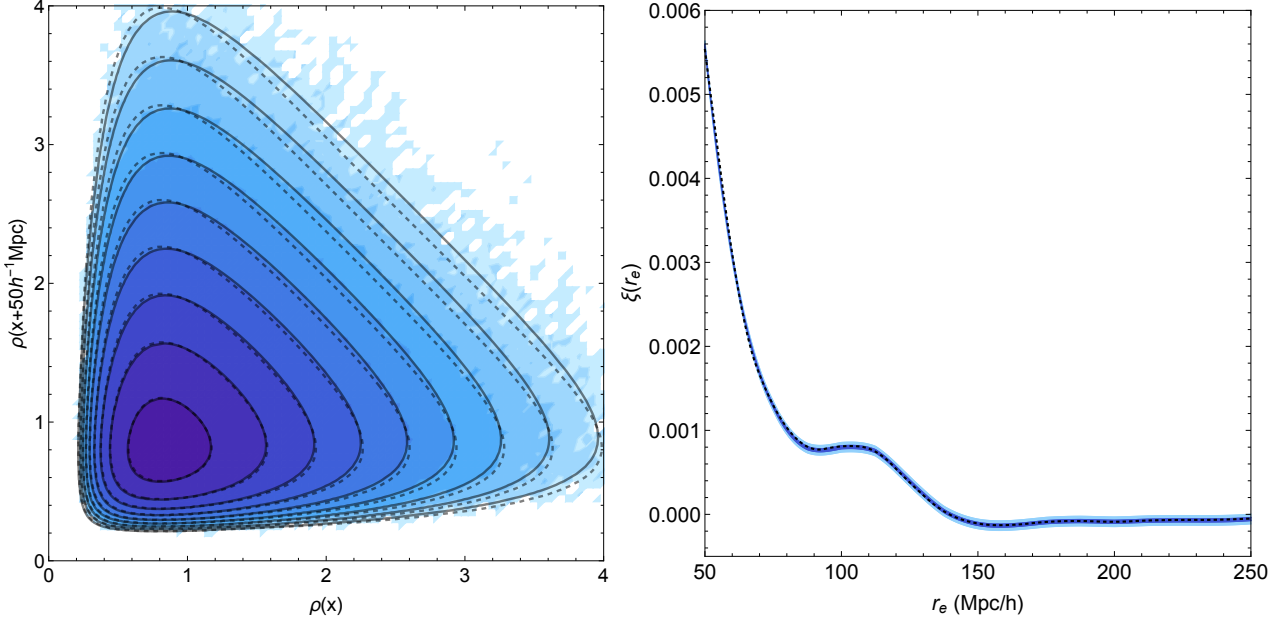
Figure 11. Left-hand panel: PDF of the densities separated by r_e = 50 \text{ Mpc}/h in the HR4 simulation (from dark to light blue) and predicted for \xi(r_e) = 0 (dashed) and 0.00558 (dotted). Contours are displayed for \log \mathcal{P} = 1, 0.5, 0 \dots -4 . Right-hand panel: one (dark blue) and three-sigma (light blue) contours for the maximum likelihood estimate of the dark matter correlation function, \hat{\xi}_{\text{ML}} , compared with the arithmetic estimate, \hat{\xi}_A , (dashed line).
