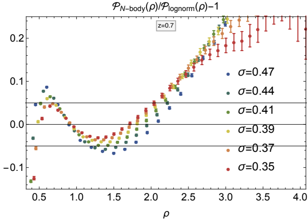
Figure D1. The residuals of the best fit log normal PDF \mathcal{P}(\rho) for redshift z = 0.7 and radii R = 10, 11, \dots, 15 \text{ Mpc/h} (from blue to red) in comparison to the measurement from HR4 (with error bars). This is to be contrasted to the quasi perfect match of the saddle PDF presented in Figure 3
