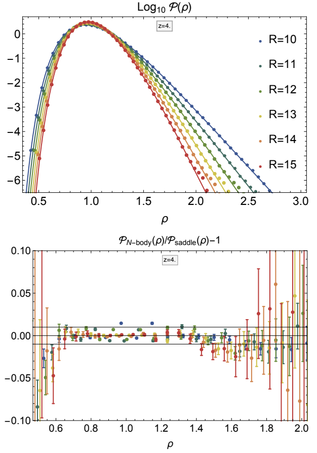
Figure D2. The density PDF \mathcal{P}(\rho) predicted from equation (23) using LSSFast (solid lines) for radii R = 10, 11, \dots, 15 \text{ Mpc/h} (from blue to red) at redshift z = 4 with \nu = 21/13 in comparison to the HR4 measurement (data points) and the corresponding residuals.
