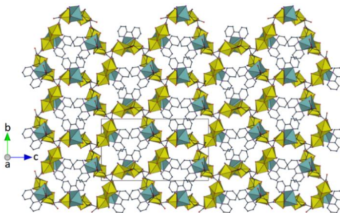
Figure 5. Top: view of complex 4 . Displacement ellipsoids are drawn at the 30% probability level and carbon-bound hydrogen atoms are omitted. Symmetry codes: i = -x, y + 1/2, 1 - z ; j = 1 - x, y - 1/2, 1 - z ; k = 1 - x, y - 1/2, -z ; l = 2 - x, y + 1/2, -z ; m = x - 1, y, z ; n = -x, y - 1/2, 1 - z ; o = 1 - x, y + 1/2, 1 - z ; p = 1 - x, y + 1/2, -z ; q = 2 - x, y - 1/2, -z ; r = x + 1, y, z . Middle: view of the uranyl citramalate anionic 3D framework. Bottom: view of the complete 3D framework. Uranium coordination polyhedra are colored yellow and those of cadmium green, and hydrogen atoms are omitted.
