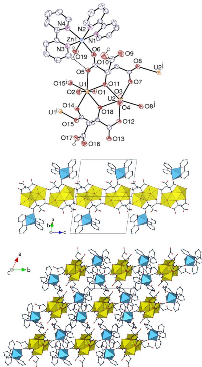
Figure 6. Top: view of complex 5 . Displacement ellipsoids are drawn at the 50% probability level. Carbon-bound hydrogen atoms are omitted and the hydrogen bond is shown as a dashed line. Symmetry codes: i = 1 - x, 1 - y, -z ; j = 1 - x, 1 - y, 1 - z . Middle: view of the 1D chain with uranium coordination polyhedra colored yellow and those of zinc blue. Bottom: view of the packing with chains viewed end-on. Hydrogen atoms are omitted in the last two views.
