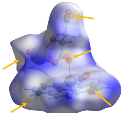
Figure 3. Hirshfeld surface mapped with d_{\text{norm}} calculated on the asymmetric unit of complex 2 . The red spots indicated by arrows correspond to the positions of CH...O hydrogen bonds. The large red dot at the top is due to truncation of the polymer chain.
