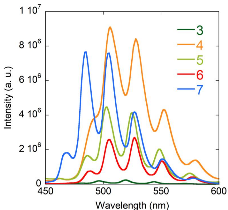
Figure 10. Solid state uranyl emission spectra of complexes 3–7 , measured with an excitation wavelength of 420 nm.
