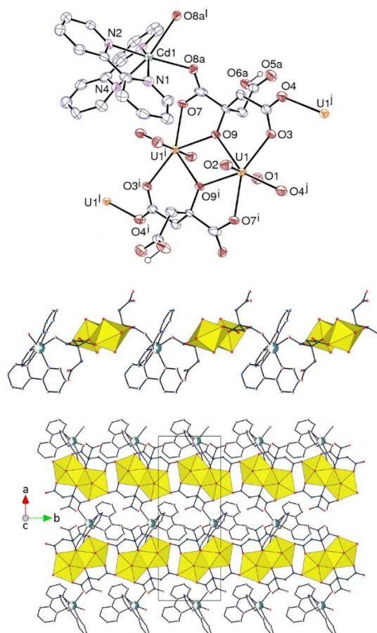
Figure 8. Top: view of complex 6 . Displacement ellipsoids are drawn at the 40% probability level. Only one position of the disordered parts is represented and carbon-bound hydrogen atoms are omitted. Symmetry codes: i = 3/2 - x , 1/2 - y , -z ; j = 3/2 - x , -y - 1/2 , -z ; l = 2 - x , y , 1/2 - z . Middle: the 2D assembly viewed edge-on, down the b axis. Bottom: the 2D assembly viewed side-on, down the c axis. Uranium coordination polyhedra are colored yellow and the disordered atoms, including cadmium, are represented as parti-coloured spheres.
