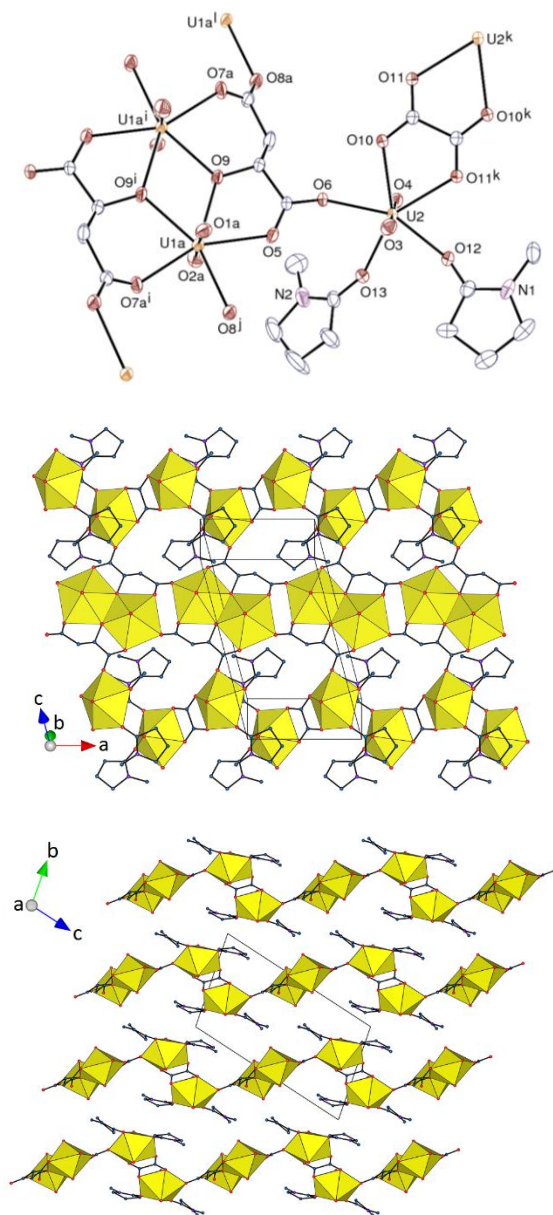
Figure 1. Top: view of complex 1 . Displacement ellipsoids are drawn at the 30% probability level. Symmetry codes: i = -x, 2 - y, 1 - z ; j = x + 1, y, z ; k = -x - 1, 1 - y, -z ; l = x - 1, y, z . Middle: view of the 2D network with uranium coordination polyhedra colored yellow. Bottom: view of the packing with sheets viewed edge-on. Only one position of the disordered atoms is represented and hydrogen atoms are omitted in all views.
