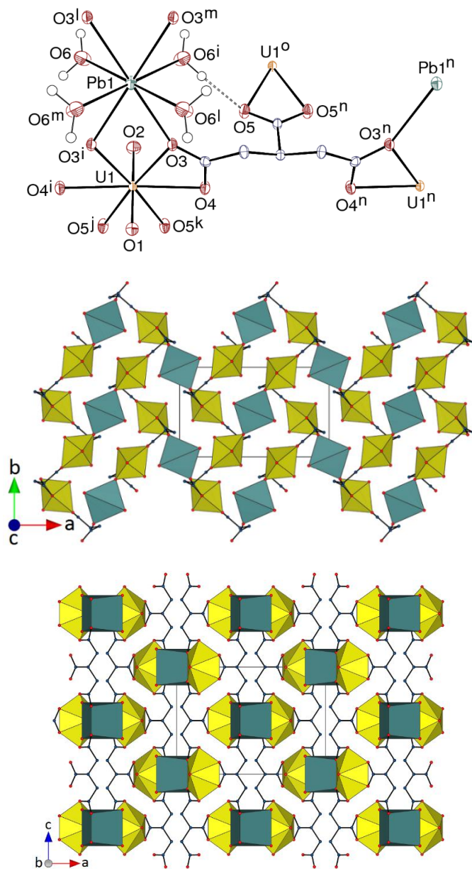
Figure 9. Top: view of complex 7 . Displacement ellipsoids are drawn at the 50% probability level. Carbon-bound hydrogen atoms are omitted and the hydrogen bond is shown as a dashed line. Symmetry codes: i = x, y, 1 - z ; j = 3/2 - x, y + 1/2, z + 1/2 ; k = 3/2 - x, y + 1/2, 1/2 - z ; l = 1 - x, 1 - y, 1 - z ; m = 1 - x, 1 - y, z ; n = x, y, -z ; o = 3/2 - x, y - 1/2, 1/2 - z . Middle and bottom: two views of the 3D framework with uranium coordination polyhedra colored yellow and those of lead green, and hydrogen atoms omitted.
