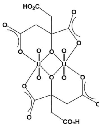
Scheme 1. The dianionic 2:2 uranyl citrate dimer involving deprotonation of the hydroxyl group and two of the three carboxylic acid groups.
