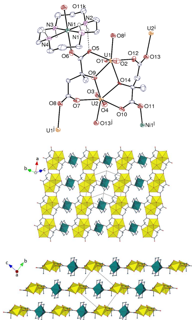
Figure 4. Top: view of complex 3 . Displacement ellipsoids are drawn at the 40% probability level. Carbon-bound hydrogen atoms are omitted and the hydrogen bond is shown as a dashed line. Symmetry codes: i = x - 1, y, z ; j = x + 1, y, z ; k = x, y + 1, z - 1 ; l = x, y - 1, z + 1 . Middle: view of the 2D network with uranium coordination polyhedra colored yellow and those of nickel green. Bottom: view of the packing with sheets viewed edge-on. Hydrogen atoms are omitted in the last two views.
