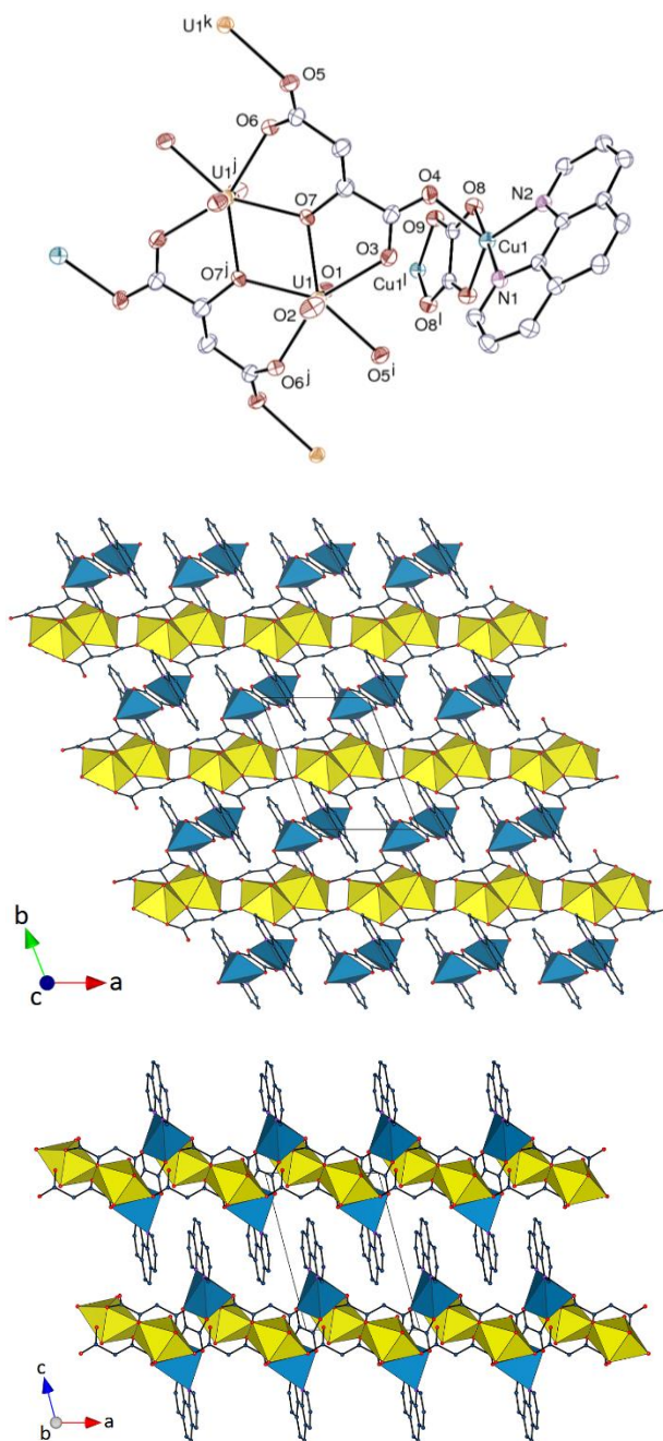
Figure 2. Top: view of complex 2 . Displacement ellipsoids are drawn at the 30% probability level. Symmetry codes: i = x - 1, y, z ; j = 1 - x, 1 - y, -z ; k = x + 1, y, z ; l = -x, -y, -z . Middle: view of the 2D network with uranium coordination polyhedra colored yellow and those of copper blue. Bottom: view of the packing with sheets viewed edge-on. Hydrogen atoms are omitted in all views.
