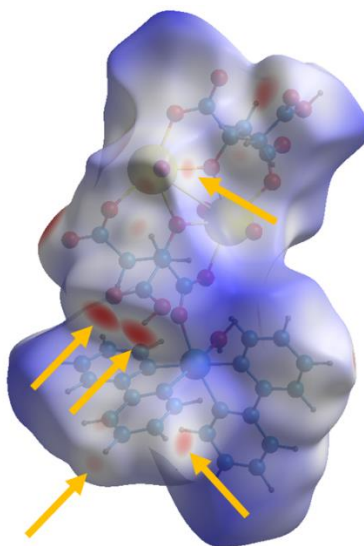
Figure 7. Hirshfeld surface mapped with d_{\text{norm}} calculated on the asymmetric unit of complex 5 . The red spots indicated by arrows correspond to the positions of OH \cdots O (between carboxylic groups, near the centre of the HS) and CH \cdots O hydrogen bonds.
