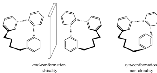
Fig. 1. Possible conformations of areno-bridged [2.4]MCPs.
