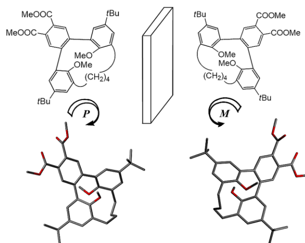
Fig. 4. Schematic diagram of M - 9 (left side) and P - 9 (right side).
