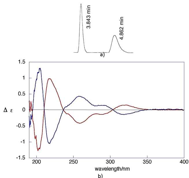
Fig. 6. (a) Chromatogram of anti -1,2-dibenzo-5,15-di- tert -butyl-8,18-dimethoxy[2.4]MCP-4',5'-dimethylcarboxylate anti - 9 (HPLC on chiral column). Daicel chiralpak ADeH. Eluent: hexanes. (b) CD spectra of P - and M -enantiomers of inherently chiral anti -1,2-dibenzo-5,15-di- tert -butyl-8,18-dimethoxy[2.4]MCP-4',5'-dimethylcarboxylate anti - 9 .
