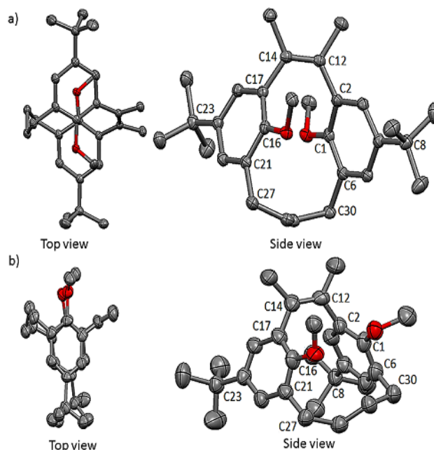
Fig. 2. Single-crystal structures of a) anti -[2.4]MCP-1-ene anti - 4 and b) syn -[2.4]MCP-1-ene syn - 4 (side view and top view). Thermal ellipsoids are drawn at the 50% probability level. All hydrogen atoms are omitted for clarity.
