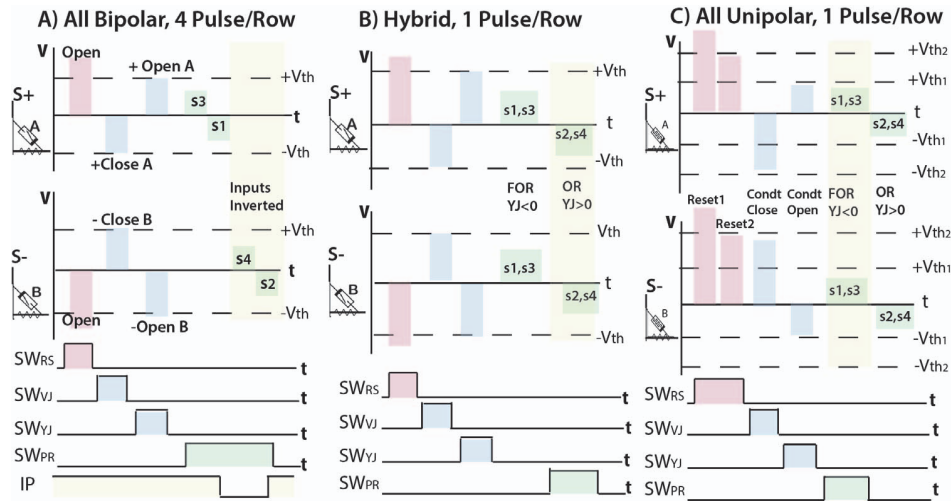
Fig. 4. A): reset, configuration, and programming scheme for bipolar devices. Altogether, 3 gate pulses, one very long gate programming pulse during which 4 individual pulses sent, and a pulse to invert inputs is required. B): hybrid approach (unipolar synapse, bipolar neuron latch) with only 4 smaller gate voltage pulses and one programming pulse required. C): all-organic scheme. It requires only three gate pulses, one programming pulse, but a slightly longer gate voltage and larger magnitude reset pulse.
