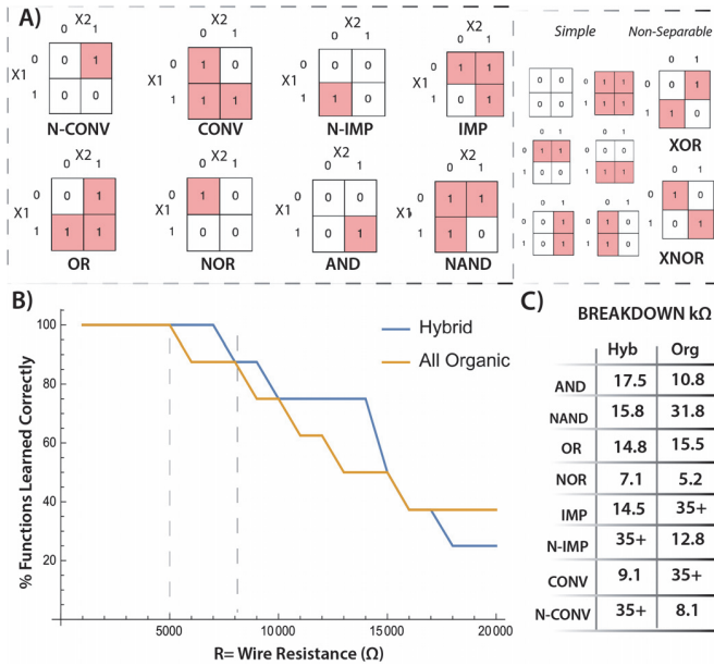
Fig. 6. A) All possible 2-bit functions. The 8 functions in the left box are the non-obvious ones on which the system is trained. B) Rate of success at learning these 8 functions for each variant system- hybrid and organic-, as a function of horizontal and vertical nanowire resistance R (40 parametric simulations), while R_{in} at the input wires is held constant at 500\Omega . C) 'Breakdown' value in R = k\Omega : the given wire resistance at which the output for one of the four cases of the truth table is incorrect.
