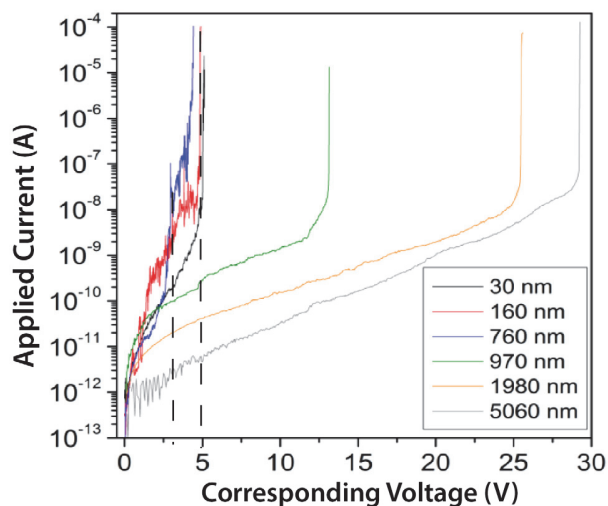
Fig. 2. Current as a function of voltage at the forming stage, measured for different device size (inter-electrode distance L ). Source: [20]
