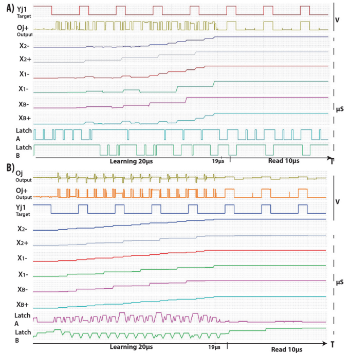
Fig. 5. A) Waveforms depicting successful learning of the AND function in the Hybrid (organic unipolar memristors, binary latch) case; target, output, 6 analog memristors being trained, and latches are depicted from top to bottom. B) Equivalent waveforms for the All-unipolar organic memristor learning case. As visible Latch behavior is now also analog.
