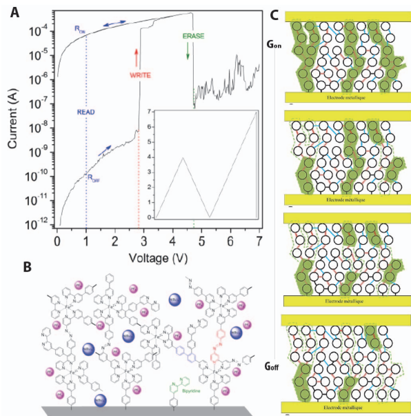
Fig. 1. A) Electrical characterization results for a single TBFe nanodevice in the positive voltage domain. Behavior in the negative voltage domain is symmetrical (flipped across the y-axis). B) Schematic of molecules that comprise the thin-film C) Filamentary development within the thin-film as current is applied between the two electrodes; conductive areas shaded in green. Source: [20]
