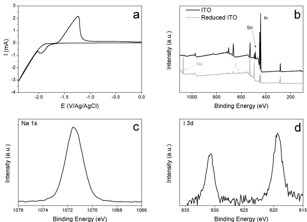
Figure 1. (a) Cyclic voltammogram recorded on ITO electrode in ACN containing 0.1 M NaI. Scan rate 0.1 \text{ V.s}^{-1} . (b) XPS survey scans of untreated ITO (black line) and reduced ITO at -2 \text{ V} in ACN containing 0.1 M NaI during 100 s (gray line). (c,d) XPS high resolution spectra for Na(1s) and I(3d).
