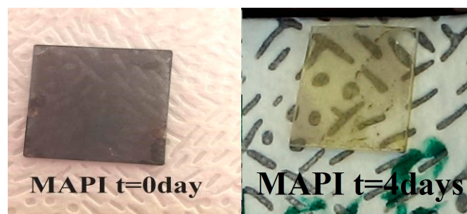
Figure 1. Photography of a 800 nm thick \text{CH}_3\text{NH}_3\text{PbI}_3 layer deposited by spin-coating on a quartz substrate, just after the deposition ( t = 0 day) and 4 days after the deposition ( t = 4 days).
