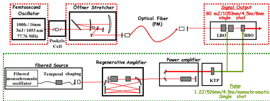
Fig. 1. Front-end schematic view.
