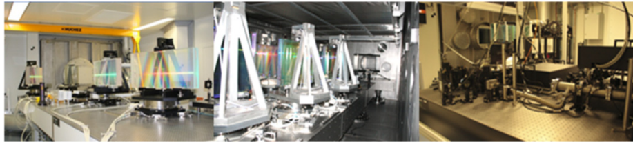
Fig. 9. 1st stage of compression in air (left), 2nd stage of compression in the vacuum vessel (center) and compression diagnostics table (right).
