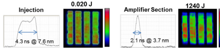
Fig. 6. Sub-apertures beam amplification up to 1.24 kJ.
