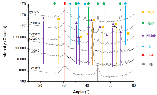
Fig. 8: XRD patterns of Ni/InP samples annealed at 250 °C, 300°C, 340°C, 350 °C, 450 °C and 550 °C for 60 seconds (RTP). A 2° offset on the incident beam was applied in order to minimize the InP substrate contribution
