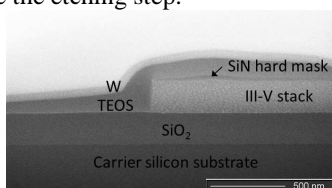
Fig. 5: FIB/SEM image of a III-V stack after its dry etching via a SiN hard mask. Note that the TEOS and W were used for the FIB etching only.
