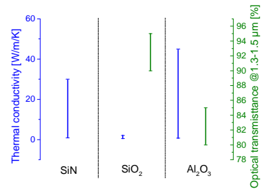
Fig. 6: Thermal conductivity and optical transmittance at 1.3-1.5 \mu\text{m} of SiN, SiO 2 and Al 2 O 3
