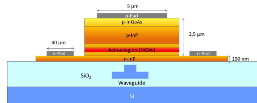
Fig. 1: Schematic representation of a III-V Laser integrated on an SOI substrate which supports the passive photonics components in the frame of Silicon Photonics
