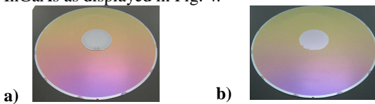
Fig. 4: Picture of a 2 inches III-V substrate (a) after its bonding to a 200 millimeters oxidized silicon substrate and (b) after the etching of the III-V carrier substrate
