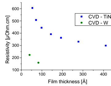
Fig. 10: Resistivity of CVD-TiN and CVD F-less W as a function of the films thicknesses
