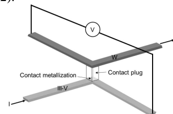
Fig. 2: Schematic representation of a cross bridge kelvin resistor (CBKR) used for the acquisition of I(V) characteristics and for specific contact resistivity extraction
