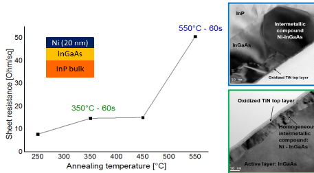
Fig. 9: Evolution of the sheet resistance in a Ni/InGaAs system after various thermal treatments and corresponding TEM pictures
