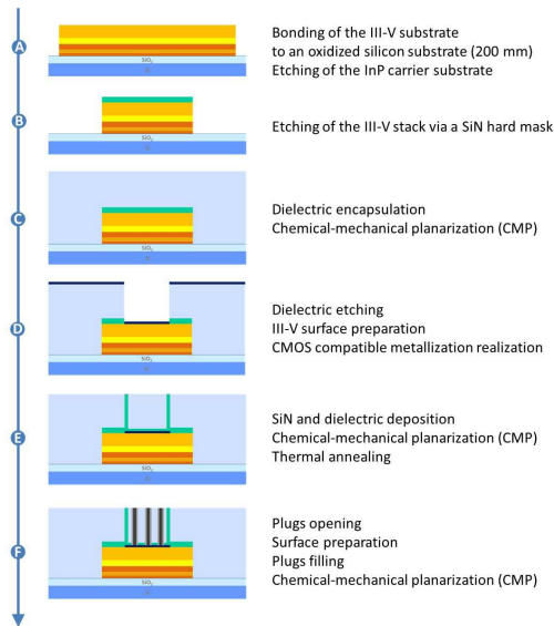
Fig. 3: CMOS compatible process flow for the integration of the contacts on a III-V epitaxy in the framework of Silicon Photonics
