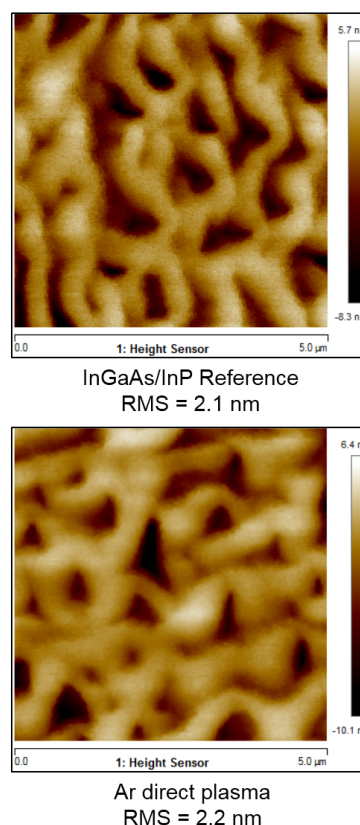
Fig. 5. AFM images for reference sample (top) and Ar direct plasma treated sample (bottom). The image space is 5 \mu\text{m} \times 5 \mu\text{m} .
