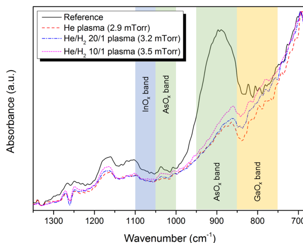
Fig. 6. Normalized FTIR-ATR spectra for InGaAs layers treated with He (red line), He/ H_2 20/1 (blue line), He/ H_2 10/1 (magenta line) plasmas and without pretreatment (black line).
