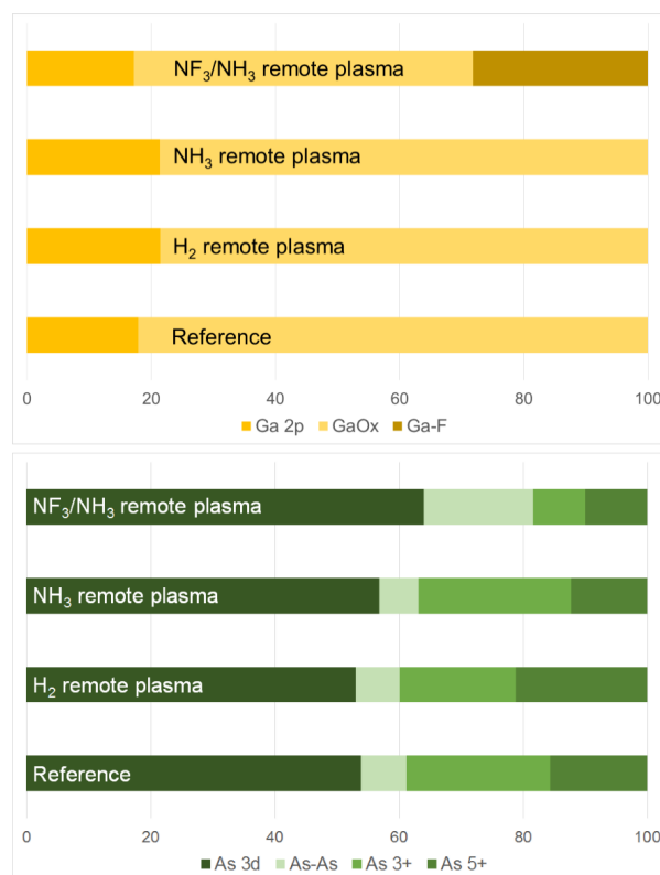
Fig. 2. Relative spectral weight of the components determined for the \text{NF}_3/\text{NH}_3 , \text{NH}_3 , \text{H}_2 remote plasma treated samples and for a reference sample for Ga 2p (top) and As 3d (bottom) regions.
