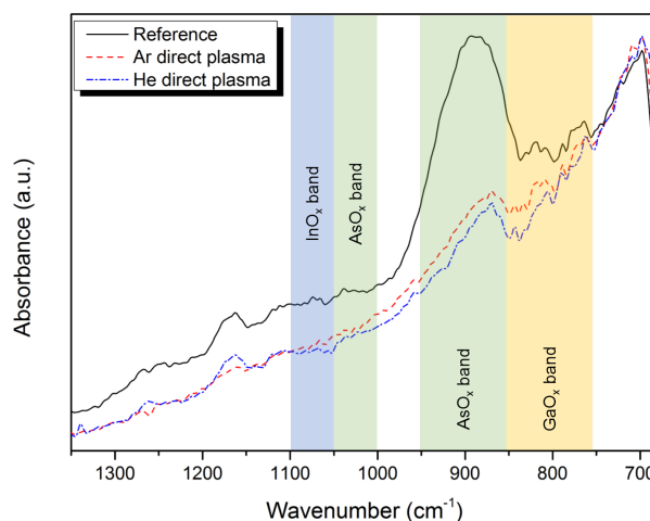
Fig. 3. Normalized FTIR-ATR spectra for InGaAs layers treated with Ar plasma (red line), He plasma (blue line) and without surface pretreatment (black line).
