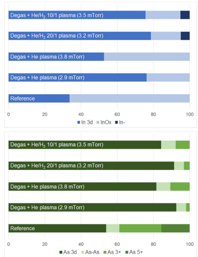
Fig. 7. Relative spectral weight of the components determined for the He-based plasma treated samples with or without addition of hydrogen and for a reference sample for In 3d (top) and As 3d (bottom) regions.
