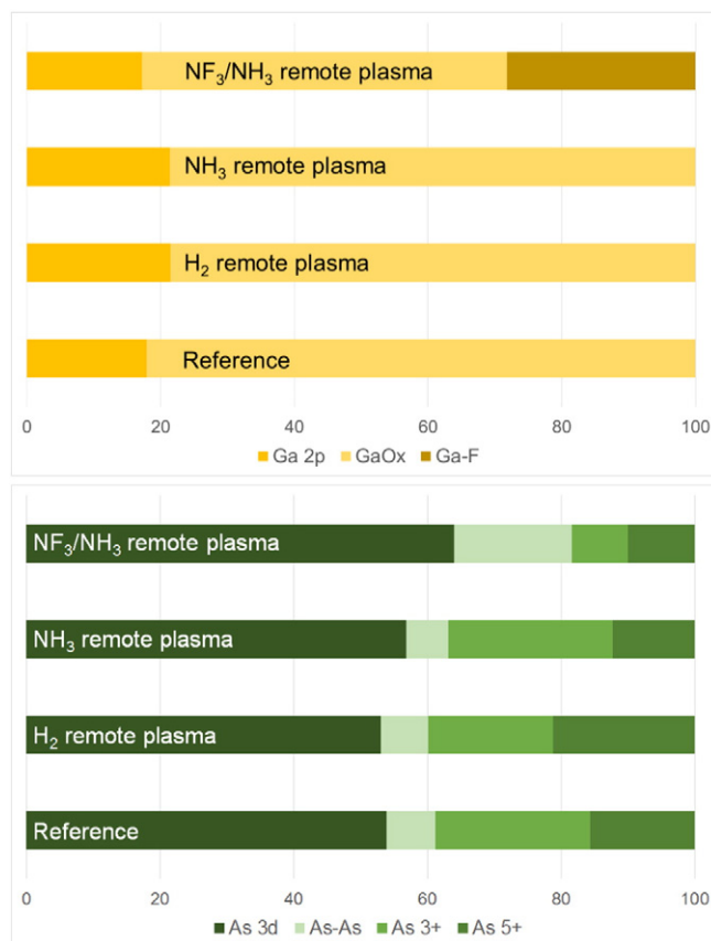
Fig. 2. Relative spectral weight of the components determined for the NF_3/NH_3 , NH_3 , H_2 remote plasma treated samples and for a reference sample for Ga 2p (top) and As 3d (bottom) regions.
