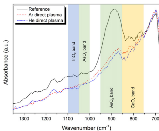
Fig. 3. Normalized FTIR-ATR spectra for InGaAs layers treated with Ar plasma (dash red line), He plasma (dash dot blue line) and without surface pretreatment (solid black line).
