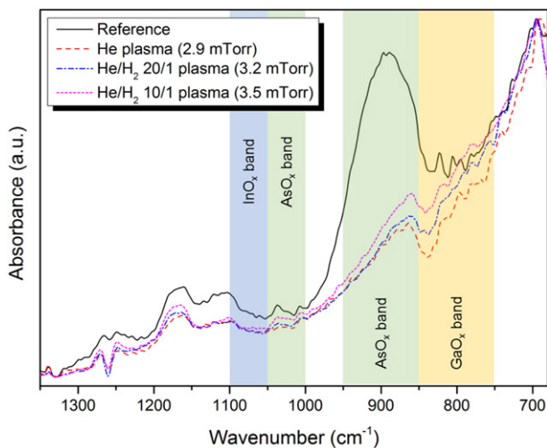
Fig. 6. Normalized FTIR-ATR spectra for InGaAs layers treated with He (dash red line), He/H 2 20/1 (dash dot blue line), He/H 2 10/1 (short dash magenta line) plasmas and without pretreatment (solid black line).
