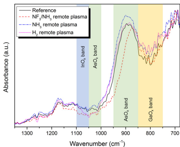
Fig. 1. Normalized FTIR-ATR spectra for InGaAs layers treated with NF_3/NH_3 (dash red line), NH_3 (dash dot blue line), H_2 (short dash magenta line) remote plasmas and without pretreatment (solid black line).
