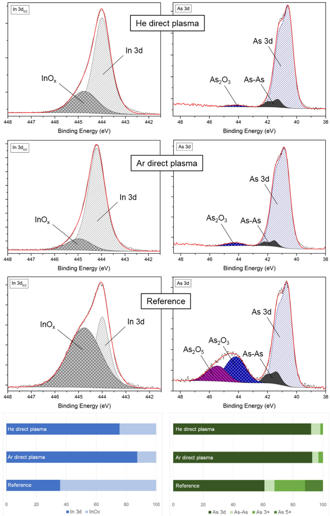
Fig. 4. XPS spectra peak fits of In 3d and As 3d regions for reference sample (bottom), Ar plasma treated sample (middle) and He plasma treated sample (top). The relative spectral weight of the components determined for the different samples is added.
