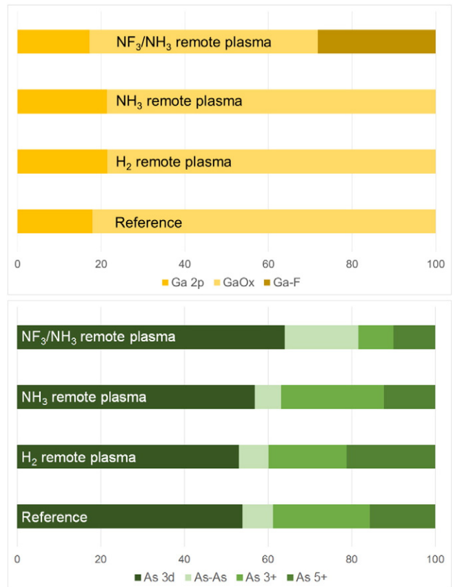
Fig. 2. Relative spectral weight of the components determined for the NF_3/NH_3 , NH_3 , H_2 remote plasma treated samples and for a reference sample for Ga 2p (top) and As 3d (bottom) regions.
