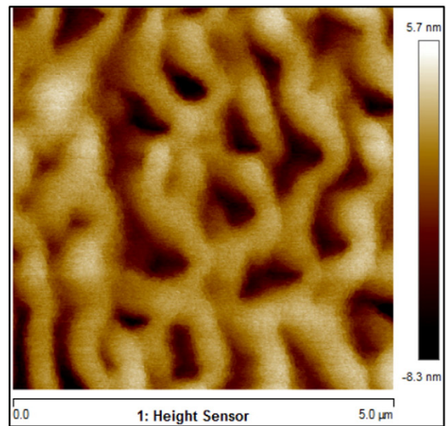
InGaAs/InP Reference RMS = 2.1 nm
