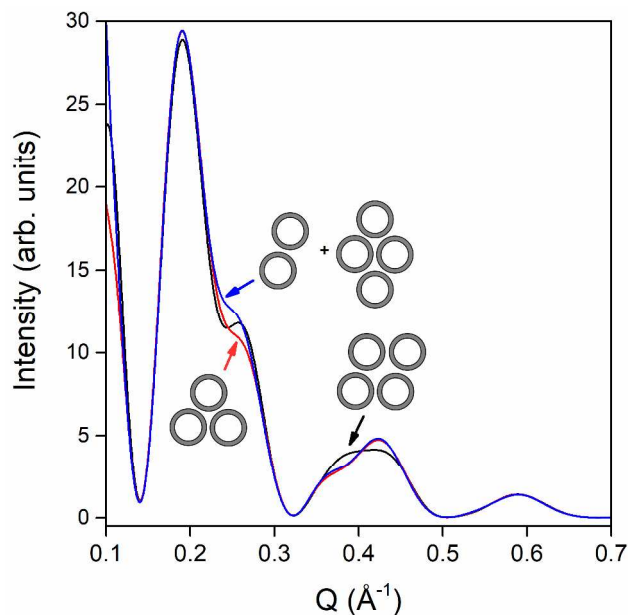
Figure 5. Calculated XRS diagrams of Ge-SWINT using eq. (5) for a monoclinic bundle (black curve, N_b = 4 , \alpha = 75^\circ ), a hexagonal bundle (red curve, N_b = 3 , \alpha = 60^\circ ) and a mixture with equal probabilities of hexagonal bundles (blue curve, N_b = 2 and 4 , \alpha = 60^\circ ).
