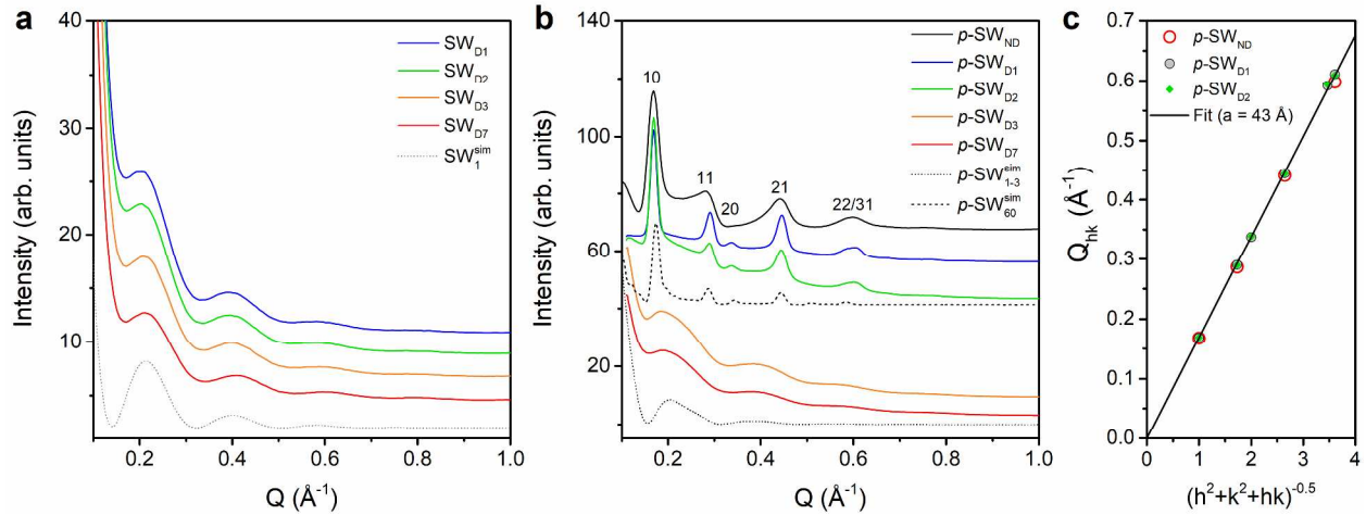
Figure 9. XRS diagrams of (a) \text{SW}_{\text{D}x} suspensions and (b) p\text{-SW}_{\text{D}x} after solvent evaporation at RT. For the sake of comparison, the XRS diagram on p\text{-SW}_{\text{ND}} sample (not dialyzed) is also represented. The hk integers index the reciprocal lattice nodes of a hexagonal 2D lattice. Dotted lines correspond to simulated XRS curves using eq. (S9) (see Supporting Information): \text{SW}_1^{\text{sim}} ( N_b = 1 ), \text{SW}_{1-3}^{\text{sim}} ( N_b = 1, p = 0.4; N_b = 2, p = 0.4; N_b = 3, p = 0.2, a = 43\text{Å} ), \text{SW}_{60}^{\text{sim}} ( N_b = 60, a = 43\text{Å} ). All curves have been translated vertically for the sake of clarity. (c) Plots of the Q vectors of the hk reflections of p\text{-SW}_{\text{D}1} & p\text{-SW}_{\text{D}2} vs. (h^2+k^2+hk)^{-0.5} . The straight line obtained from eq. (7) illustrates the good agreement of the peak positions with a 2D hexagonal packing of the lattice parameter a = 43 \text{Å} .
