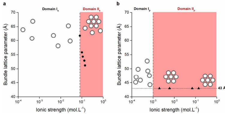
Figure 10. Phase diagrams (ionic strength/lattice parameter a ) obtained for Ge-SWINT in (a) aqueous suspensions and (b) after solvent evaporation in dry state. Circle symbols correspond to the bundle lattice parameter obtained in aqueous suspensions while black triangles are related to those obtained in dry state. INT sketches represent the different Ge-SWINT organizations, deduced from XRS experiments and simulations.
