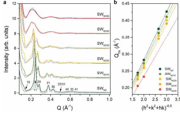
Figure 8. (a) Evolution of XRS diagrams of SW_{NDy} suspension upon the dilution ratio y . Solid curves: experimental measurements; dotted curves: calculated XRS diagrams (see text for details). In both cases, the XRS curves have been translated vertically for the sake of clarity. (b) Plots of the Q values of the hk reflections vs. (h^2+k^2+hk)^{-0.5} . The dotted lines obtained from eq. (7) illustrate the 2D hexagonal packing and allow one to determine the lattice parameter a .
