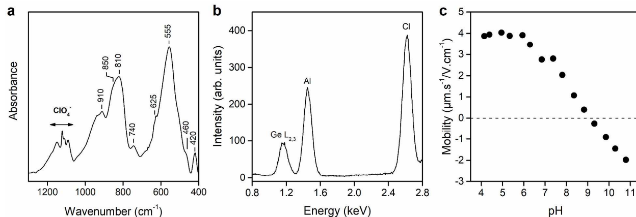
Figure 6. (a) Infrared and (b) X-Ray fluorescence spectra obtained on the SW D7 powder. (c) Electrophoretic mobility of a dilute SW D7 suspension (0.1% w/v) as a function of the pH.
