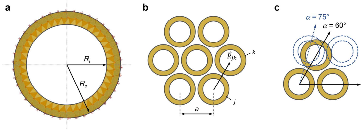
Figure 3. Schematic representations of: (a) a single-walled nanotube, in the homogeneous approximation, perpendicularly to its long axis; (b) nanotubes arranged on a 2D hexagonal lattice drawn in the plane perpendicular to the tubes axes; (c) hexagonal vs. monoclinic packing configuration.
