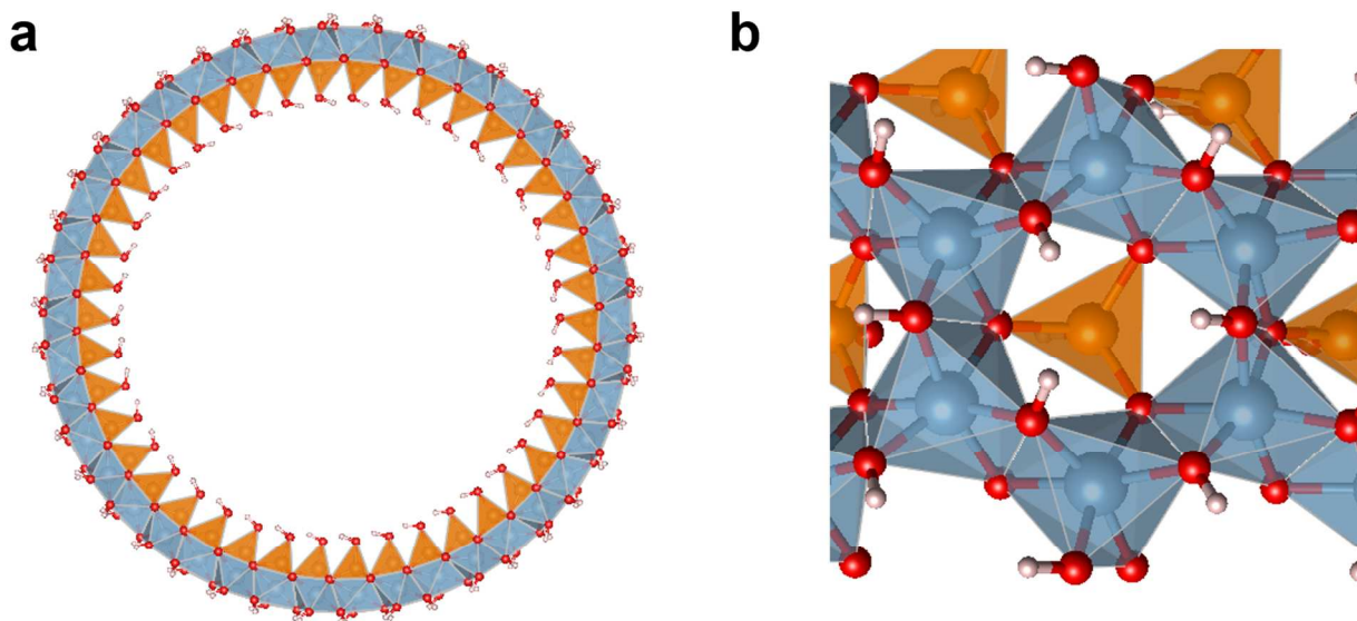
Figure 1. (a) Top and (b) side view of a single-walled imogolite nanotube. Al: blue; Si/Ge: orange; O: red; H: white.
