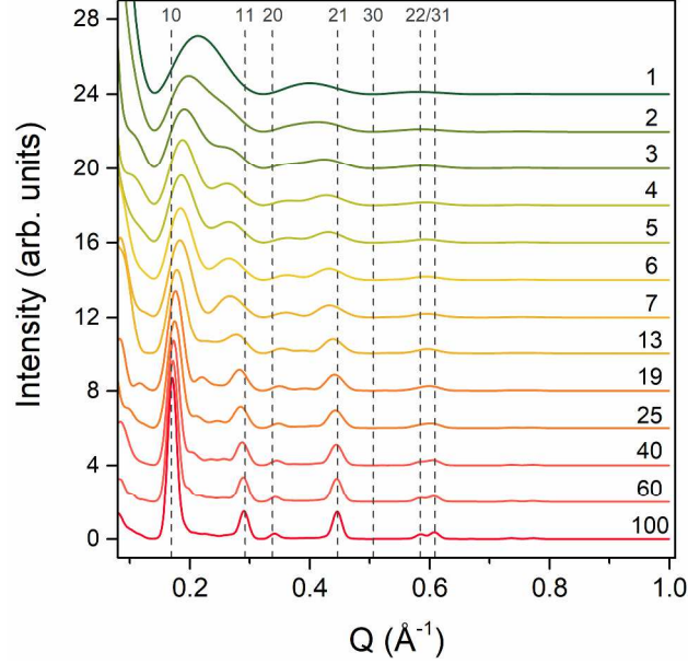
Figure 4. Simulated XRS diagrams for suspensions of bundles formed by N_b tubes in hexagonal packing ( a = 43 \text{\AA} ). N_b values, from 1 to 100, are indicated in the figure. The hk integers (dotted lines) index the reciprocal lattice nodes of an infinite hexagonal 2D lattice given in eq. (7). XRS curves have been translated vertically for the sake of clarity.
