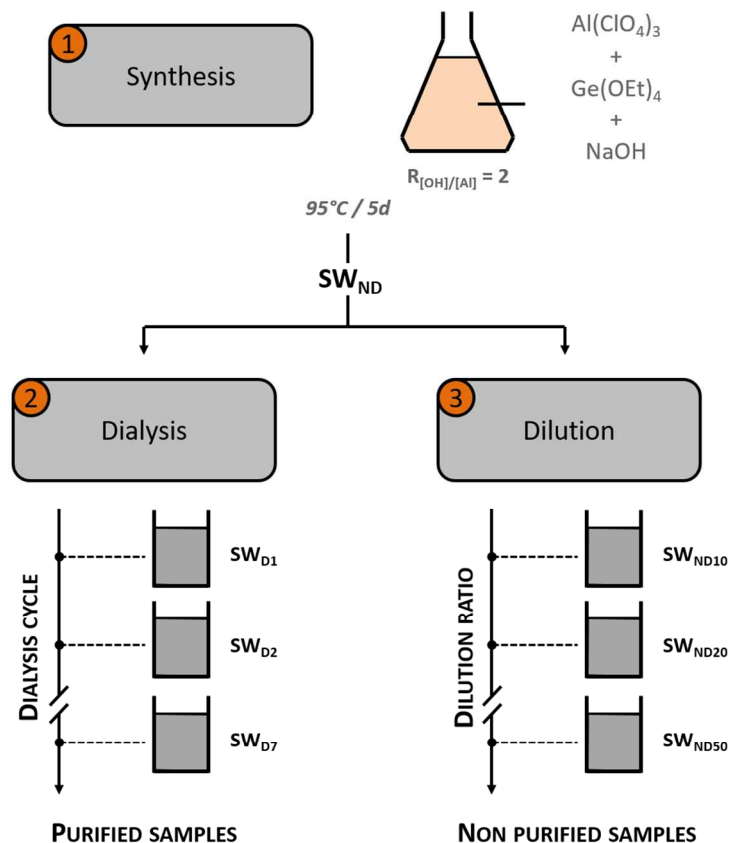
Figure 2. Flowchart for the synthesis of Ge-SWINT and samples preparation used in this study.
