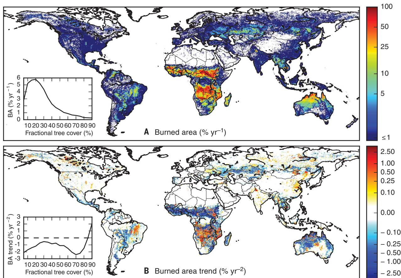
Fig. 1. Satellite observations show a declining trend in fire activity across the world's tropical and temperate grassland ecosystems and land-use frontiers in the Americas and Southeast Asia. (A) mean annual burned area and (B) trends in burned area (GFED4s, 1998 through 2015). Line plots (inset) indicate global burned area and trend distributions by fractional tree cover (28).
