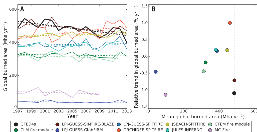
Fig. 3. Comparison of burned area trends from satellite observations (GFED4s) and prognostic fire models from FireMIP. (A) Time series of global burned area. (B) A comparison of global mean annual burned area versus the relative trend in global mean burned area from the observations and models. GFED4s observations are shown in black and FireMIP models are shown with different colors. FireMIP model estimates were available from 1997 through 2013 for six models, from 1997 through 2012 for the CTEM fire module and JULES-INFERN0, and from 1997 through 2009 for MC-Fire. The FireMIP models are described in more detail in the supplementary materials and by Rabin et al. (34) (tables S3 and S4 and fig. S8).
