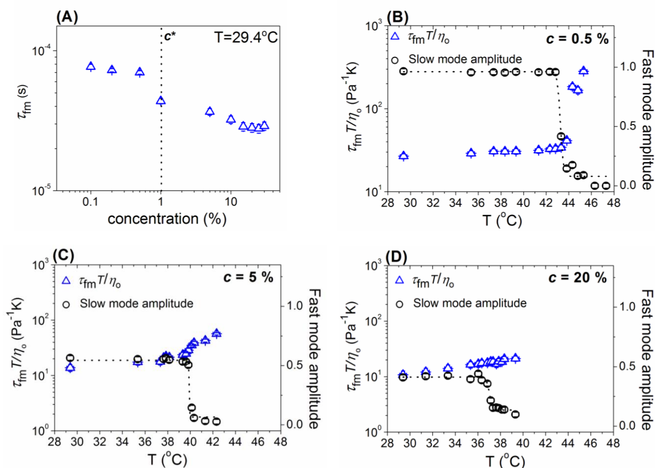
Figure 3. (a) Fast mode relaxation time vs. concentration in the single phase region at 29.4^\circ\text{C} and normalized fast mode relaxation time ( \tau_{fm} T / \eta_0 ) vs. T for concentrations (b) 0.5 %, (c) 5 % and (d) 20 %.
