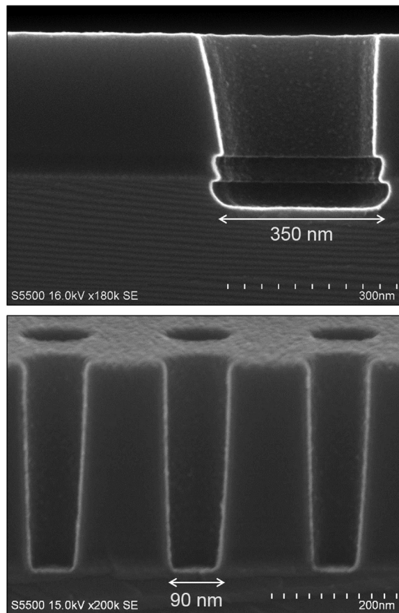
Fig. 9. SEM observations of two contact structures cross section after F-free W film deposition. Due to the contrast used, the W film appears in bright on these SEM pictures.
