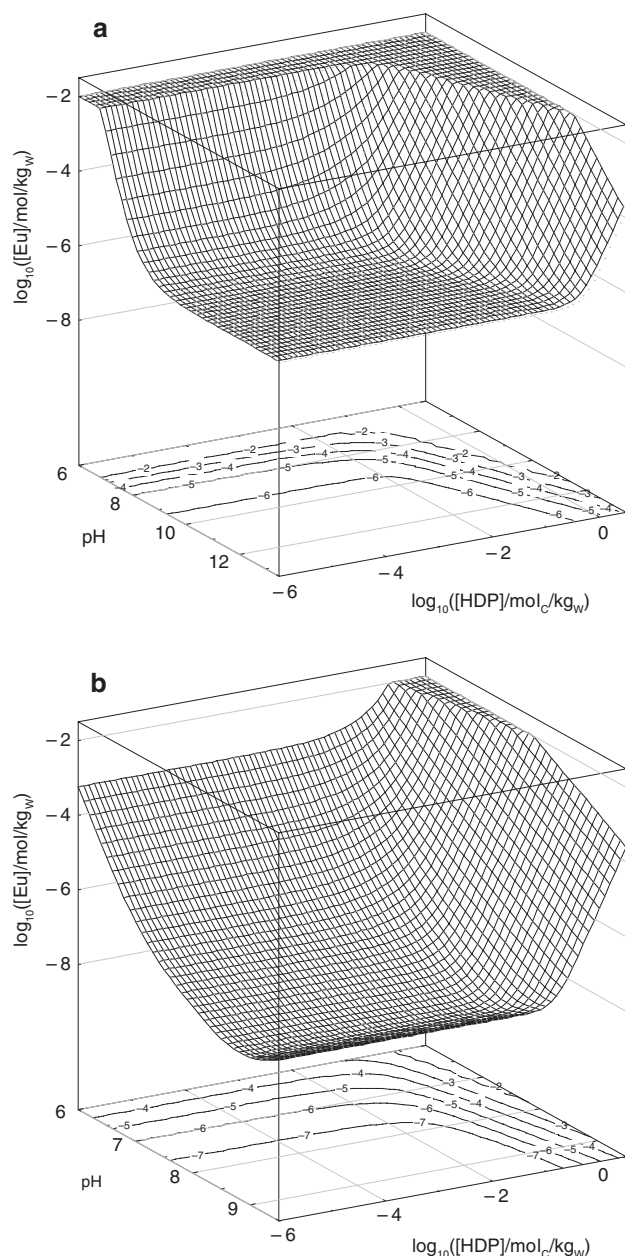
Figure 5: Evolution of the solubility surfaces of [Eu]_{\text{tot}} = 10^{-2} \text{ mol/kg}_w as a function of pH and concentration of \gamma -PVC-HDP, on total carbon basis, using thermodynamic constants [23, 25] and formation constants for \text{Eu(OH)(HDP)} and \text{Eu(OH)}_2(\text{HDP})_3 in Table 2 of (a) \text{Eu(OH)}_3(\text{am}) at \text{PCO}_2(\text{g}) = 10^{-12} \text{ atm} , and (b) \text{EuOHCO}_3(\text{cr}) at \text{PCO}_2(\text{g}) = 10^{-3.5} \text{ atm} .
