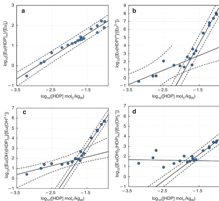
Figure 3: Determination of the Eu(III)-HDP complexes' stoichiometries – on \text{mol}_C/\text{kg}_W basis – and apparent formation constants K_{op} from TRLS results from Figure 2 considering (a) total non-complexed europium, (b) \text{Eu}^{3+} free, (c) \text{EuOH}^{2+} , and (d) \text{Eu}(\text{OH})_2^+ in solution using hydrolysis constants [23]; [\text{Eu}(\text{III})]_{\text{total}} = 10^{-6} \text{ mol}/\text{kg}_W , I = 0.1 \text{ M NaCl} .
