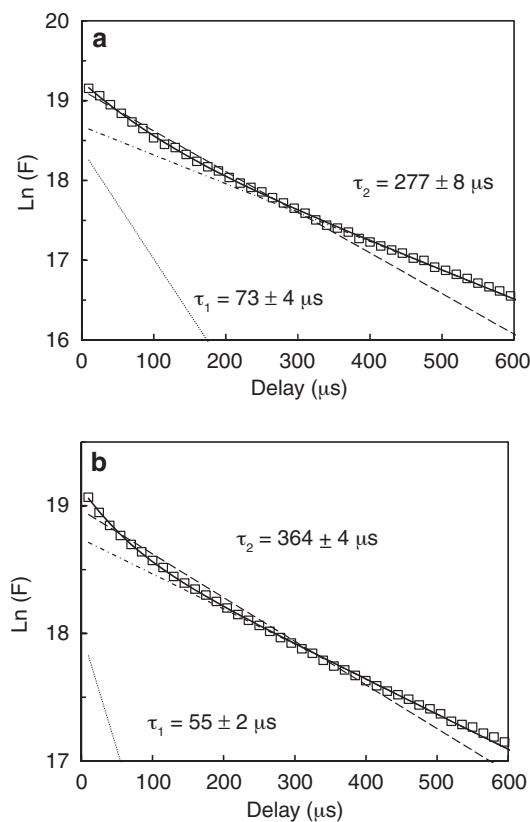
Figure 4: Luminescence decays of Eu(III) at (a) 0.021 \text{mol}_\text{c}/\text{kg}_\text{w} (pH 8.85, \log_{10}([\text{HDP}]/\text{mol}_\text{c}/\text{kg}_\text{w}) = -1.68 ) and (b) 0.274 \text{mol}_\text{c}/\text{kg}_\text{w} (pH 11.21, \log_{10}([\text{HDP}]/\text{mol}_\text{c}/\text{kg}_\text{w}) = -0.56 ) of \gamma -PVC-HDPs. Calculated on the area of the ^5\text{D}_0 \rightarrow ^7\text{F}_2 transition, W = 300 \mu\text{s} , \lambda_{\text{exc}} = 393.7 nm; plain line is the bi-exponential decay composed of a fast (dotted) and a slow (dash-dot) component, and dashed line is the mono-exponential decay. Uncertainties on decay times are fitting uncertainties.
