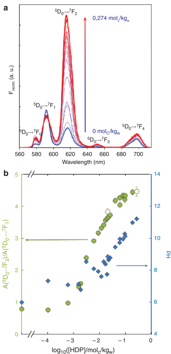
Figure 2: Evolutions with the \gamma -PVC-HDPs concentration ( \text{mol}_c/\text{kg}_w ) of (a) the luminescence spectra of Eu(III) normalized to the area of the ^5\text{D}_0 \rightarrow ^7\text{F}_1 transition – from 0 blue thick line to 0.274 \text{ mol}_c/\text{kg}_w red thick line –, and (b) the ^7\text{F}_2/^7\text{F}_1 asymmetry ratio (circles) and solution pH (diamonds); [\text{Eu}] = 1 \mu\text{M} , D = 10 \mu\text{s} , W = 300 \mu\text{s} , \lambda_{\text{exc}} = 393.7 \text{ nm} , I = 0.1 \text{ M NaCl} ; empty circles represent experiments for which decay time measurements are presented in Figure 4. Error bars represent 2\sigma of the ^7\text{F}_2/^7\text{F}_1 asymmetry ratio using the trapezoid method.
