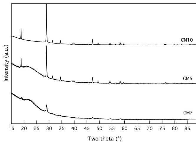
Fig. 5. XRD patterns of \text{CaMoO}_4 bearing samples in the M series.
