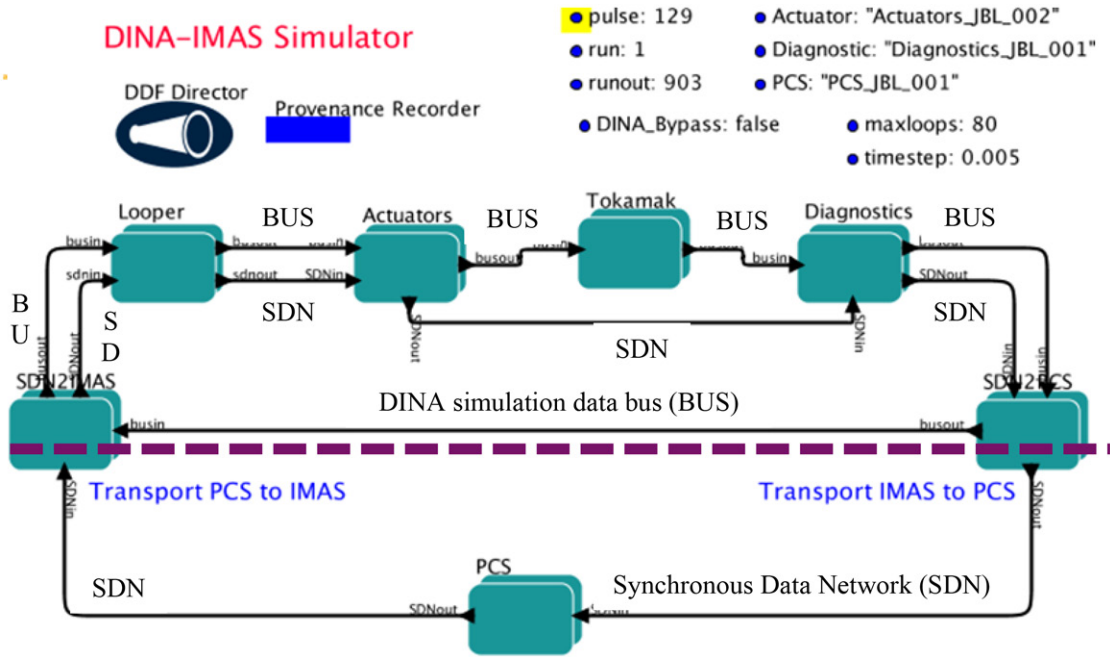
Figure 6. Overview of the implemented DINA-IMAS simulator (workflow designed and executed using the Kepler workflow engine), highlighting the coupling between the various elements of the full tokamak simulator: actuators, tokamak, diagnostics, plasma control system (PCS). The boxes correspond to high level components of the workflow and contain themselves more detailed sub-workflows. The arrows connecting the boxes represent the data flow, which consists of two main streams: the DINA simulation data bus (BUS), which stays on the IMAS side, and a representation of the ITER SDN, which is the interface between the PCS and the plant.
