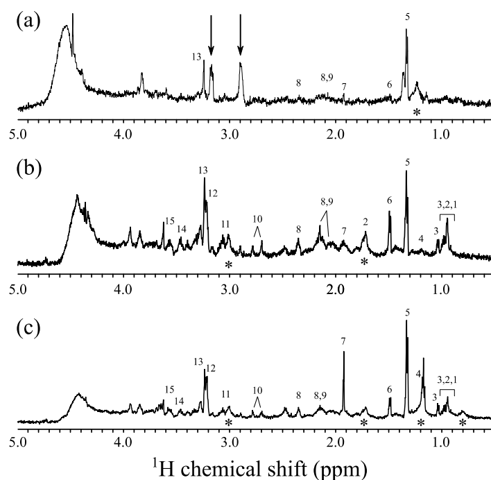
Figure 3. Proton 1D spectra of methanol treated (a) and untreated (b,c) neurosphere samples. All experiments were recorded by Carr–Purcell–Meiboom–Gill (CPMG) sequence with the total echo delay of 1.0 ms. The experimental times were from 15 to 20 h. The asterisk (*) denotes the lipid peak. The detailed assignments are given in Table 1.
