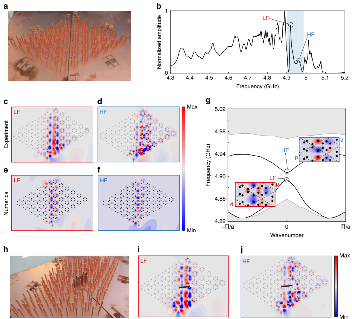
Figure 4 | Experimental observation of topological edge modes guided at the subwavelength scale. (a) We form a boundary between the topologically trivial sample and the topologically nontrivial one. (b) Spectrum of the field amplitude measured in the sample, averaged along the boundary. Two peaks appear in the band gap corresponding to a low frequency (LF) and a high frequency edge mode (HF). (c,d) Experimental electric field maps for the LF and HF edge modes. (e,f) Corresponding field maps computed from a coupled-dipole semi-analytical model. (g) Corresponding dispersion diagram for the edge modes, shown in inserts. (h) We insert a defect in the form of a large conducting wall placed right on the boundary. (i,j) Measured electric field maps in the presence of a defect, showing good robustness of the edge modes despite the breaking of sixfold rotational symmetry along the interface.
