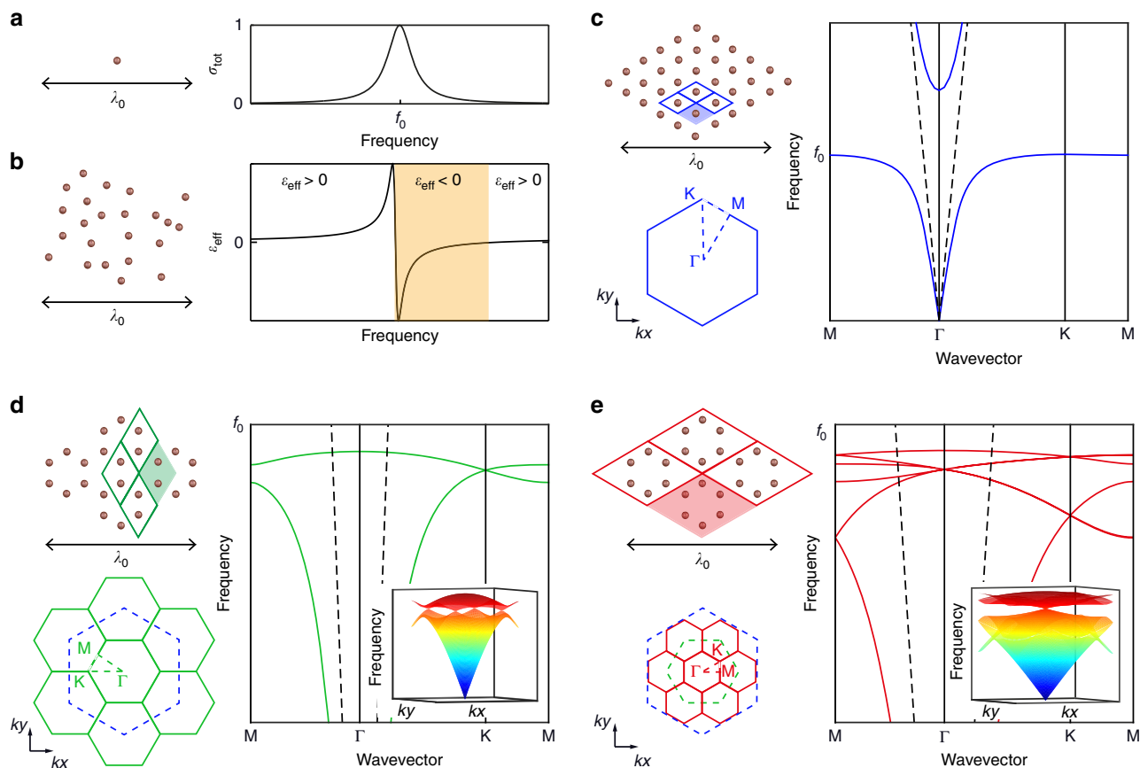
Figure 1 | Subwavelength band structure engineering in resonant metamaterials. (a) A subwavelength resonator and its scattering cross-section. (b) A dense two-dimensional ensemble of subwavelength resonators with arbitrary structure makes a metamaterial with negative permittivity (orange band) after the individual resonance of the resonators. Here the resonators are quarter wavelength copper rods sitting on a ground plane. (c) By adding a periodic subwavelength structure, in the form of a triangular array, such a metamaterial can acquire crystalline properties, involving a Bloch band structure with typical polaritonic dispersion corresponding to subwavelength bound modes localized to the array of rods. (d) More complex crystalline properties can be obtained, including point Dirac degeneracy at K point, by considering the polaritons supported by a honeycomb metamaterial. (e) Same lattice as c but viewed in the extended unit cell picture, allowing for mathematical folding of two time-reversed Dirac cones at the \Gamma point. These two time-reversed degenerate states are exploited here as the equivalent of Kramers pairs to induce topological properties at the subwavelength scale.
