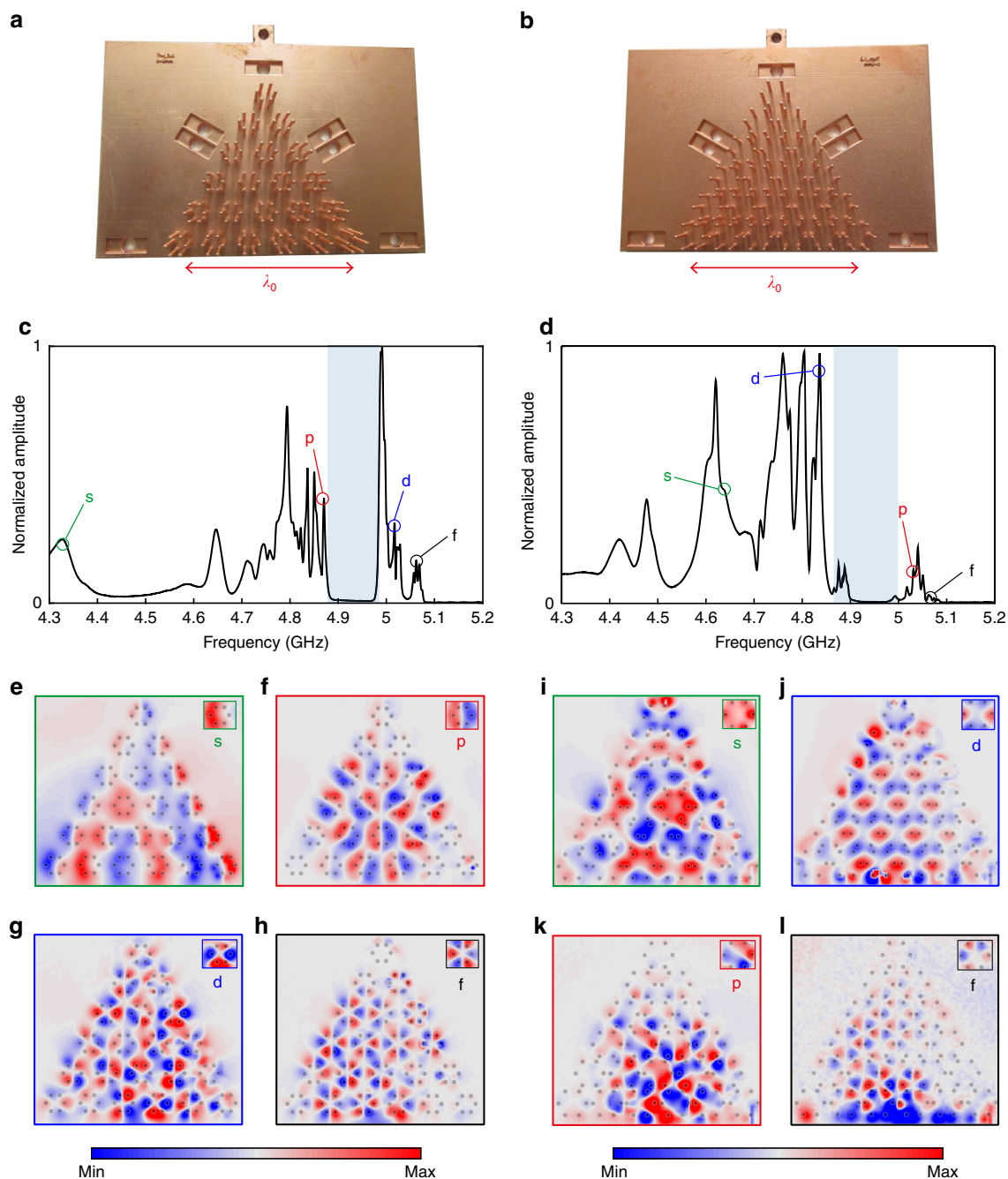
Figure 3 | Experimental validation of subwavelength, topologically nontrivial phases. We have fabricated by 3D printing followed by chemical metallization two subwavelength sized samples composed of conducting rods on a ground plane. (a) Picture of the topologically trivial sample made of shrunk hexagons. (b) Picture of the topologically nontrivial sample made of expanded hexagons. (c) Electric field amplitude spectrum in the bulk of the topologically trivial sample (spatially averaged). A complete band gap is observed (shaded frequency range). Outside of this gap, peaks correspond to efficient excitation of s , p , d and f type bulk Bloch modes, as confirmed by the electric field maps at these frequencies (e,f,g,h) . (d) Same as (c) for the topologically nontrivial sample, demonstrating the topological band inversion phenomenon induced by subwavelength structural deformations, with the order of appearance of the p and d bands reversed with respect to the band gap. (i,j,k,l) Same as (e,f,g,h) for the topologically non-trivial sample.
