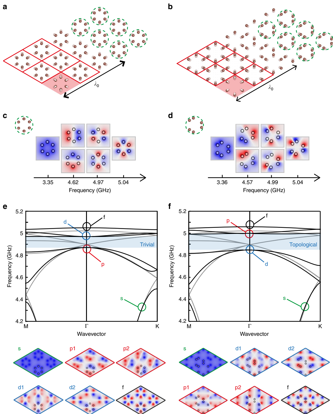
Figure 2 | Opening of a topological band gap by subwavelength structural modifications. (a) Starting from the honeycomb lattice in the extended unit cell picture of Fig. 1e, we shrink the size of the hexagonal arrangement of resonators composing each unit cell, obtaining a triangular lattice of hexagonal metamolecules (circled in green). Conversely, in (b) we expand the size of the hexagons, obtaining an array composed of a different metamolecule involving a trimer of resonator pairs (circled in green). (c,d) The resonant modes of the two metamolecules, responsible for the six bands observed in the band structures of the two crystals (e,f). (e) The band structure of the lattice of shrunken hexagons, and the associated electric field distribution for the Bloch modes of the six bands at the \Gamma point. (f) Similar to (e) for the lattice of extended hexagons, except that the p and d bands are now inverted with respect to the bandgap. As demonstrated in the text, the bandgap (blue shaded area) in (e) is topologically trivial, whereas the one in (f) is associated with a non-trivial topology.
