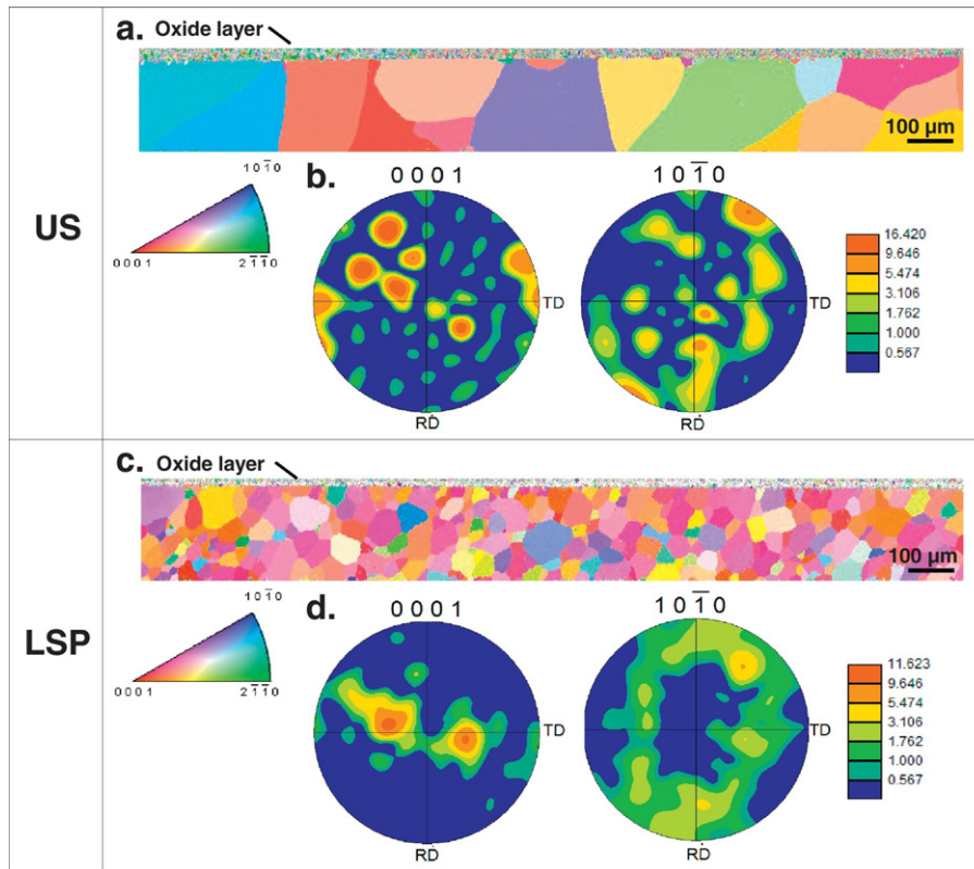
Fig. 8. EBSD results obtained after 10 h of oxidation at 700 °C in dry air for (a,b) US and (c,d) LSP samples. (a,c) Maps (2000 × 250 μm 2 ) of grain orientation (HCP structure). (b,d) Direct-pole figures.
