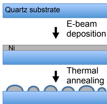
Fig. 1. Scheme of the synthesis process. A thin Ni layer is deposited by e-beam evaporator in vacuum then this layer is annealed at low pressure.
