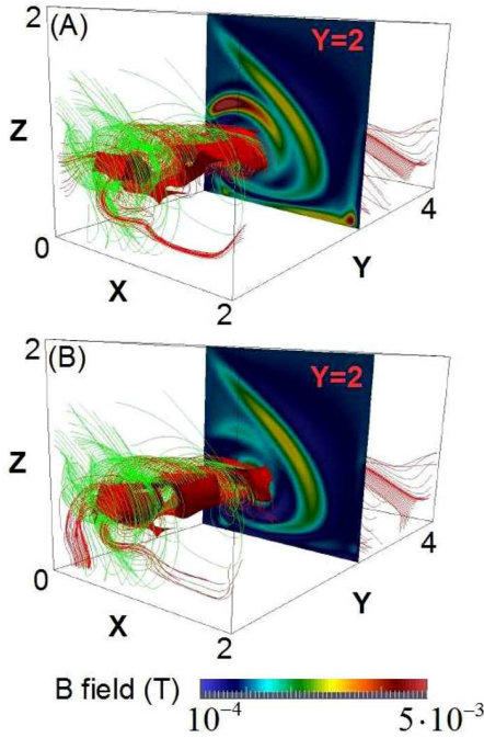
FIG. 6. Magnetic (red line) and velocity field streamlines (green line) for simulations with R_e = 200 , \Gamma = 0.8 and Bx orientation of the remnant magnetic field in the FerroCond30 (a) and CondFerro30 (b) cases. Isocontour of the magnetic field module of 0.00125 T (red). Contour plot of the magnetic field module in the Y = 2 plane.
