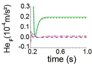
FIG. 9. Kinetic helicity of the fluctuations (solid green line) and current helicity of the fluctuations (dashed red line) for the FerroCond30 case, as well as the kinetic helicity of the fluctuations (dotted blue line) and current helicity of the fluctuations (dash-dotted pink line) for the CondFerro30 case. (Simulations with R_e = 200 and \Gamma = 0.8 ).
