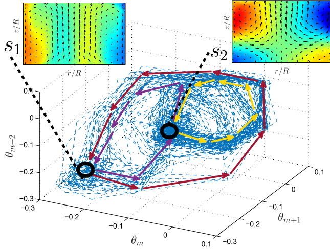
FIG. 2. The von Kármán turbulent flow attractor reconstructed for the experiment performed at \gamma = 0.067 . The attractor is obtained by embedding the peaks \theta_m extracted from the time series \theta(t) in a three-dimensional space. One can identify two quasistationary states (labeled as s_1 and s_2 ) corresponding to the average velocity fields (dark red insets, arrows, and color scale show, respectively, the in-plane and the orthogonal average velocity and three cycles (highlighted by colored arrows). The direction of the arrows indicates the only possible paths to switch from one state to the other. See also Supplemental video [19].
