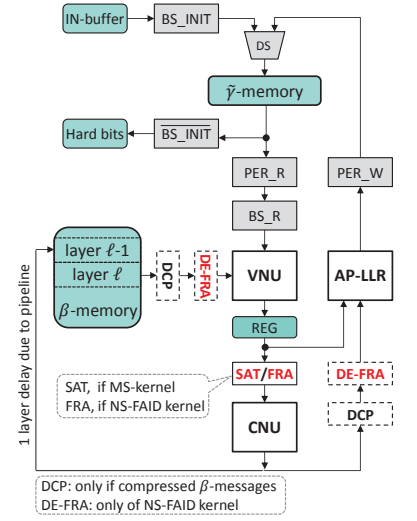
(b) High-Level Description of the HW Architecture with MS and NS-FAID kernels
