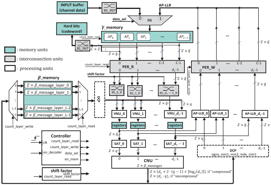
(a) Detailed HW Architecture with MS-kernel
