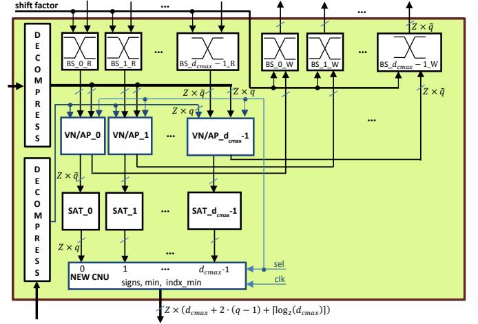
Figure 3. New processing units for the layered MS decoder architecture
