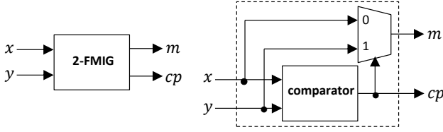
Figure 7. 2-FMIG architecture
