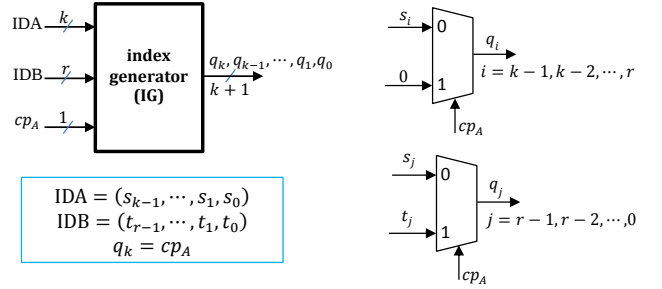
Figure 9. IG (Index Generator) architecture
