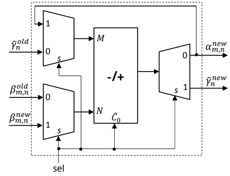
Figure 4. VNU/AP-LLR processing unit
