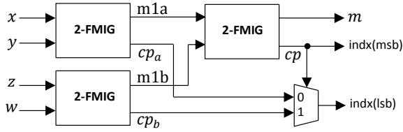
Figure 8. 4-FMIG architecture
