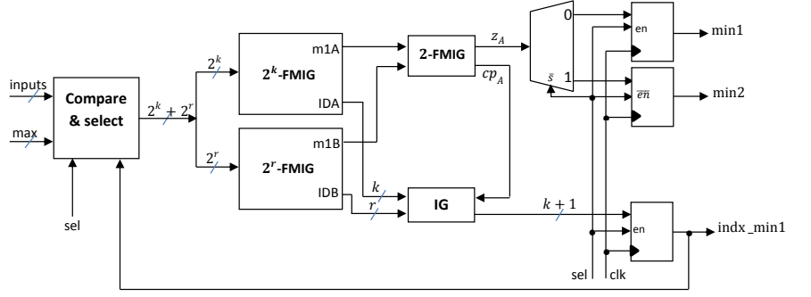
Figure 6. Block diagram of the proposed CNU architecture
