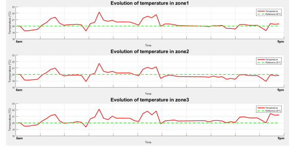
Fig. 5. Indoor temperature in the three zones, Centralized MPC
