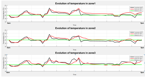
Fig. 7. Indoor temperature in the three zones, centralized (black) and distributed (red) control schemes
