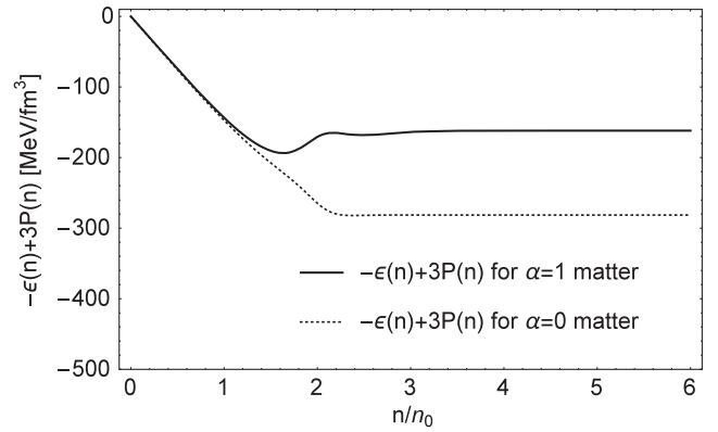
FIG. 4. -\epsilon(n) + 3P(n) vs density for \alpha = 0 and \alpha = 1 .
