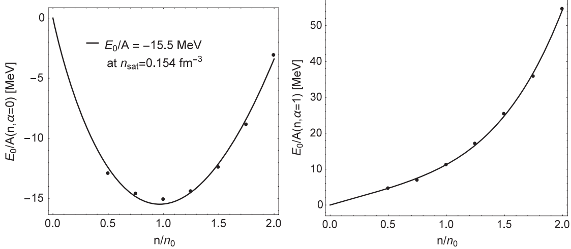
FIG. 1. E_0/A for \alpha = 0 (left) and \alpha = 1 (right) matter, where \alpha = (N_n - N_p)/A and A = N_n + N_p with the proton/neutron number N_p/n . The dots are from the V_{\text{lowk}} RG and the solid lines are fit by Eq. (45). The saturation density is estimated as n_{\text{sat}} = 0.154 \text{ fm}^{-3} .
