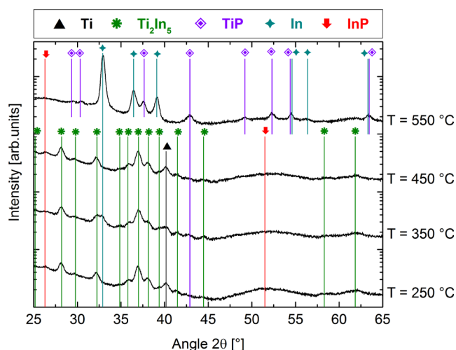
FIG. 4. XRD detexturation patterns of the TiN (7 nm)/Ti (20 nm)/InP samples annealed at 250, 350, 450, and 550 °C for 60 s (RTP). A 2° offset on the incident beam was applied in order to minimize the InP substrate contribution.
