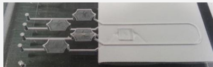
Microfluidic device with on-line measurement sites.
