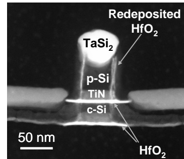
FIGURE 11. HAADF STEM image of lamella B of fig. 10.
