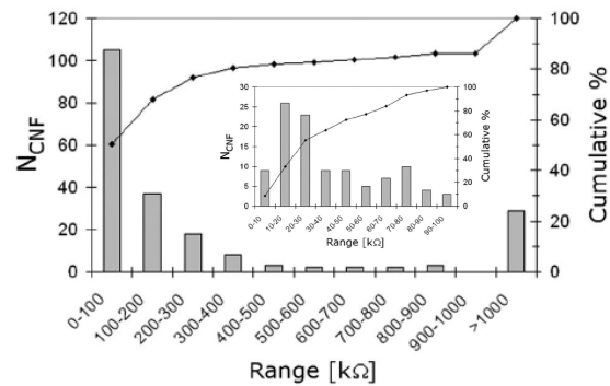
FIGURE 7. SPMs in contact mode on embedded vertical CNF: statistical analysis of the SSRM measurement performed on about 200 CNFs after calibration and conversion of the SSRM signal in resistance units [26].
