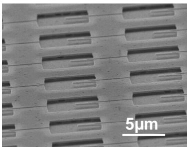
FIGURE 18. SEM view of NEMS array manufactured in a VLSI scheme
