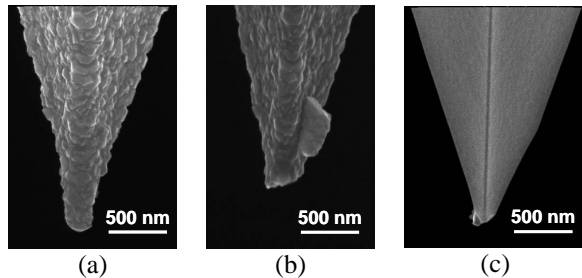
FIGURE 9. SEM observation of SPM tip: (a) Diamond coated Si tip before use; (b) Diamond coated Si tip and (c) PtIr coated Si tip after SSRM measurements.
