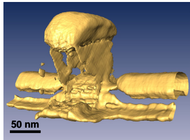
FIGURE 12. Reconstructed 3D image from HAADF STEM tilt series of the device of figure 10.
