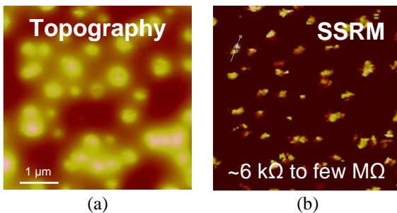
FIGURE 6. SPMs in contact mode on embedded vertical CNF: (a) AFM topography (amplitude range of about 300 nm), (b) SSRM measurement using a PtIr coated silicon tip (brightest points in the electrical image correspond to the more conductive CNF).
