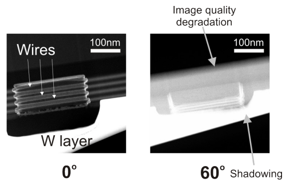
FIGURE 14. NWs device TEM tomography imaging: Two views of the TEM image series acquired for tomography.
