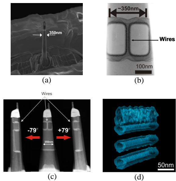
FIGURE 15. Needle shaped specimen for reliable 3D TEM tomography on integrated NWs: (a) SEM view of the FIB prepared needle; (b) HAADF STEM image showing the vertically aligned NWs in the needle; (c) extreme angle images of the tilt series (d) Iso-surface representation of NWs device showing boundaries of TiN layers.
