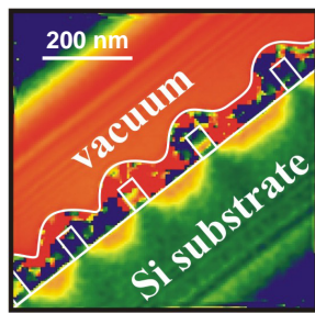
FIGURE 3. Reconstructed phase image in false colors obtained using off-axis electron holography on 45 nm CMOS structures thanks to a controlled sample thickness on a wide field of view and the TEM stability.
