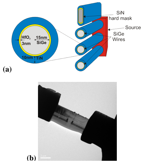
FIGURE 13. NWs device TEM tomography imaging (a) Nanowire schematic structure; (b) SEM view of the lamella sample preparation.
