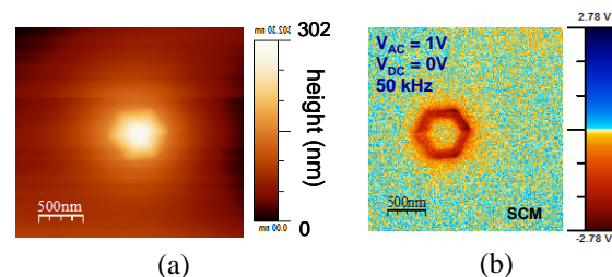
FIGURE 8. ZnO nanowire embedded in polymer: (a) AFM topography; (b) SCM measurement using a PtIr coated silicon tip.
