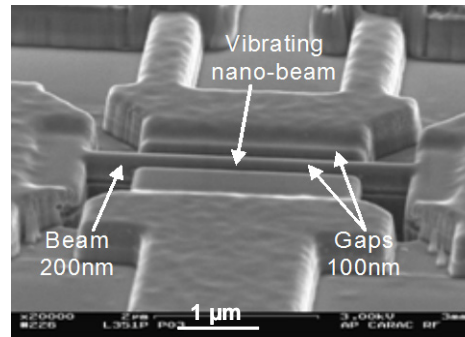
FIGURE 16. SEM view of a clock time reference radio frequency NEMS with high aspect ratio features.
