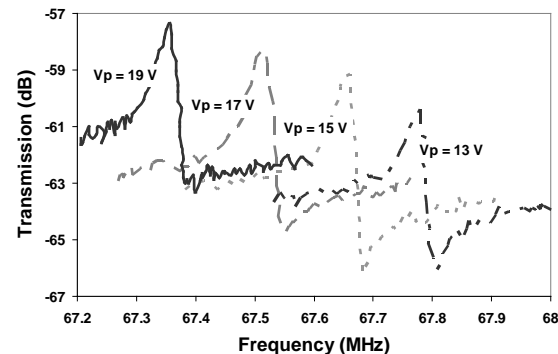
FIGURE 17. Dynamical characterization using capacitive detection of the clock time reference radio frequency NEMS of figure 16.
