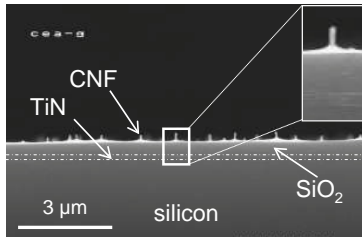
FIGURE 5. SEM view of CNF embedded in SOG to allow SPM electrical measurements.
