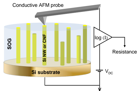
FIGURE 4. Scheme of the electrical SPM characterization of as grown vertical nanomaterials SSRM configuration used for local electrical characterization
