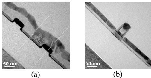
FIGURE 10. 2D images bright field TEM of a complex device inducing a TEM sample lamellae with in-depth heterogeneous structure: (a) lamella A and (b) lamella B (lamellae A and B are perpendicular to each other, lines added to the bright field image of lamella A indicate the position of the lamella B).
