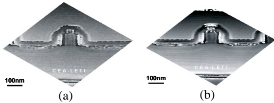
FIGURE 2. Reconstructed phase image obtained using off-axis electron holography on a CMOS device with an integration time of (a) 4s and (b) 45s thanks to the column stability of the FEI Titan microscope and a well controlled TEM environment.
