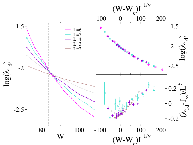
FIG. 5: Left panel: \lambda_{1d} as a function of the disorder W for several system sizes L from 2 to 6. The vertical dashed line spots the position of the critical point, W_c \simeq 83.5 . Top-right panel: Finite size scaling of the same data for L equal to 4, 5 and 6, showing data collapse for \nu \simeq 0.84 . Bottom-right panel: \psi f_1 = (\lambda_{1d} - f_\infty)/L^y as a function of the scaling variable (W - W_c)L^{1/\nu} for different sizes L from 2 to 5, showing data collapse for the same value as before of W_c and \nu for y \simeq -1.4 .
