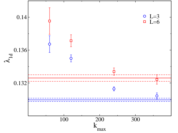
FIG. 12: Quasi- 1d dimensionless localization length, \lambda_{1d} , obtained using the SDRG procedure for different values of k_{\max} , at the AL critical point, W_c \simeq 83.5 , in 6 dimensions, and for L = 3 (blue circles) and L = 6 (red squares). The horizontal blue (resp., red) solid and dashed lines corresponds to the average value of \lambda_{1d} and its fluctuations computed using the TM method for L = 3 (resp., L = 6 ), showing that for k_{\max} \gtrsim 240 the approximate SDRG results converge, within our numerical accuracy, to the exact values.
