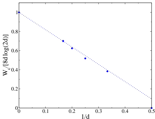
FIG. 16: Dimensional dependence of the critical value of the disorder strength, W_c , divided by 8d \log(2d) , which corresponds to the exact asymptotic behavior on tree-like lattices in the large connectivity limit [55]. The straight dotted blue line is a fit that takes into account corrections in 1/d , from which we find: W_c/8d \log(2d) \simeq 1 - 1,81/d .
