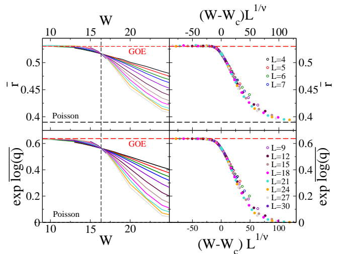
FIG. 6: \bar{r} (top-left) and q^{typ} (bottom-left) as a function of the disorder W for several system sizes L from 4 to 30. The horizontal dashed lines correspond to the reference GOE and Poisson asymptotic values. The vertical dashed line spots the position of the AL transition, W_c \simeq 16.35 . Finite size scaling of the same data (top and bottom-right panels) showing data collapse obtained for \nu \simeq 1.57 . Finite-size corrections to Eq. (12) are observed at small sizes (open symbols), and can be described by Eq. (10) with y \simeq -1 .
