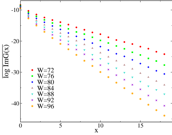
FIG. 2: \overline{\log \text{Im}G(x)} as a function of x in 6 dimensions, for L = 6 and for several values of the disorder, showing that \xi_{1d} can be measured from Eq. (6) by linear fitting of the data at large enough x .
