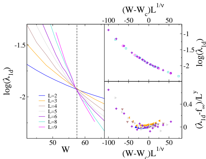
FIG. 4: Left panel: \lambda_{1d} as a function of the disorder W for several system sizes L from 2 to 9. The vertical dashed line spots the position of the critical point, W_c \simeq 57.5 . Top-right panel: Finite size scaling of the same data for L from 6 to 9, showing data collapse for \nu \simeq 0.96 . Bottom-right panel: \psi f_1 = (\lambda_{1d} - f_\infty)/L^y as a function of the scaling variable (W - W_c)L^{1/\nu} for different sizes L from 2 to 6, showing data collapse for the same value as before of W_c and \nu for y \simeq -1.2 .
