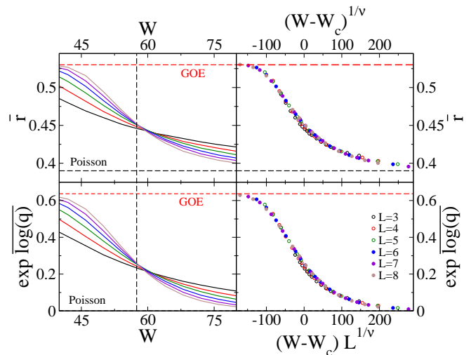
FIG. 8: \bar{r} (top-left) and q^{typ} (bottom-left) as a function of the disorder W for several system sizes L from 3 to 8. The horizontal dashed lines correspond to the reference GOE and Poisson asymptotic values. The vertical dashed line spots the position of the AL transition, W_c \simeq 57.5 . Finite size scaling of the same data (top and bottom-right panels) showing data collapse obtained for \nu \simeq 0.96 . Finite-size corrections to Eq. (12) are observed at small sizes (open symbols), and can be described by Eq. (10) with y \simeq -1.2 .
