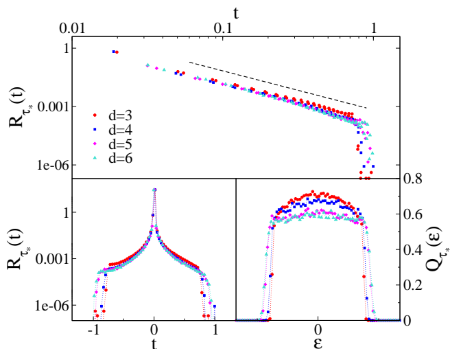
FIG. 13: Bottom-left and bottom-right panels: The stationary distributions R_{\tau_*}(t) and Q_{\tau_*}(\epsilon) at the AL critical points in dimensions from 3 to 6. The system size is L = 33 in 3d , L = 14 in 4d , L = 8 in 5d , and L = 6 in 6d , in such a way that the total number of sites is approximately the same, N \sim 4 \cdot 10^4 , in all dimensions. The stationary state is reached for a RG time \tau_* such that the number of sites left in the system are approximately 1/8 of the initial ones in 3d , 1/16 in 4d , 1/26 in 5d , and 1/40 in 6d . The value of k_{\max} is set to 360 in all dimensions. Top-panel: The same data of the bottom-left panel plotted in a log-log scale, showing the power law behavior of R_{\tau_*}(t) \sim t^{-\gamma} with \gamma \simeq 2 (black dashed line), for t smaller than a cut-off of O(1) .
