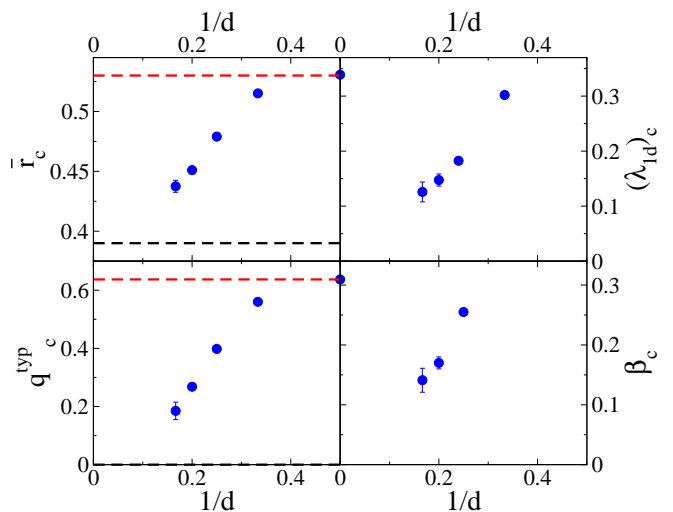
FIG. 15: Dimensional dependence of \bar{r}_c (top-left panel), q_c^{typ} (bottom-left panel), (\lambda_{1d})_c (top-right panel), and \beta_c at the AL critical point as a function of 1/d . The dashed horizontal red (resp. black) lines correspond to the reference GOE (resp. Poisson) values.
