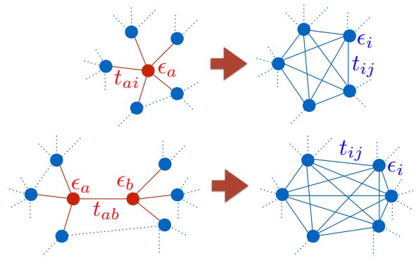
FIG. 11: Sketch of the SDRG decimation procedure for a site (top), and a bond (bottom) transformation. Dotted blue lines represent pre-existing hopping amplitudes before decimation. Solid blue lines represent new or renormalized bonds. The on-site energies of all the neighbors of the decimated sites (blue circles) are renormalized as well.
