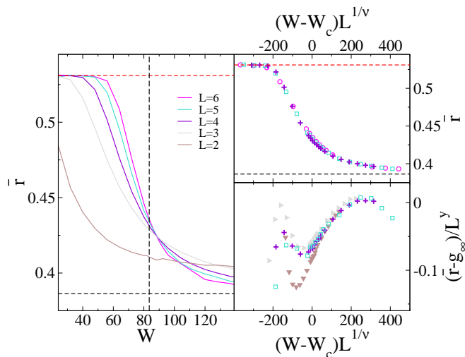
FIG. 9: Left panel: \bar{r} as a function of the disorder W for several system sizes L from 2 to 6. The horizontal dashed lines correspond to the reference GOE and Poisson asymptotic values. The vertical dashed line spots the position of the AL transition, W_c \simeq 83.5 . Top-right panel: Finite size scaling of the same data for the largest system sizes only, L = 4, 5 , and 6 , showing data collapse for \nu \simeq 0.84 . Bottom-right panel: \psi g_1 = (\bar{r} - g_\infty)/L^y as a function of the scaling variable (W - W_c)L^{1/\nu} for different sizes L from 2 to 5, showing a reasonably good data collapse for the same value as before of W_c and \nu , and for y \simeq -1.4 .
