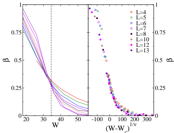
FIG. 10: Left panel: Flowing fractal exponent \beta describing the scaling of the typical value of the IPR with the system size. The vertical dashed black line corresponds to the critical disorder W_c \simeq 34.5 . Right panel: Finite size scaling of the same data showing a reasonably good data collapse obtained for \nu \simeq 1.11 . Strong finite-size corrections to the one-parameter scaling are observed at small sizes (open symbols), and can be described by Eq. (10) with y \simeq -1 .
