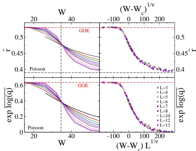
FIG. 7: \bar{r} (top-left) and q^{typ} (bottom-left) as a function of the disorder W for several system sizes L from 3 to 13. The horizontal dashed lines correspond to the reference GOE and Poisson asymptotic values. The vertical dashed line spots the position of the AL transition, W_c \simeq 34.5 . Finite size scaling of the same data (top and bottom-right panels) showing data collapse obtained for \nu \simeq 1.11 . Finite-size corrections to Eq. (12) are observed at small sizes (open symbols), and can be described by Eq. (10) with y \simeq -1 .
