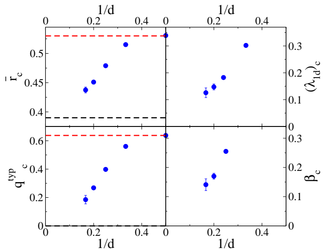
FIG. 15: Dimensional dependence of \bar{r}_c (top-left panel), q_c^{typ} (bottom-left panel), (\lambda_{1d})_c (top-right panel), and \beta_c at the AL critical point as a function of 1/d . The dashed horizontal red (resp. black) lines correspond to the reference GOE (resp. Poisson) values.
