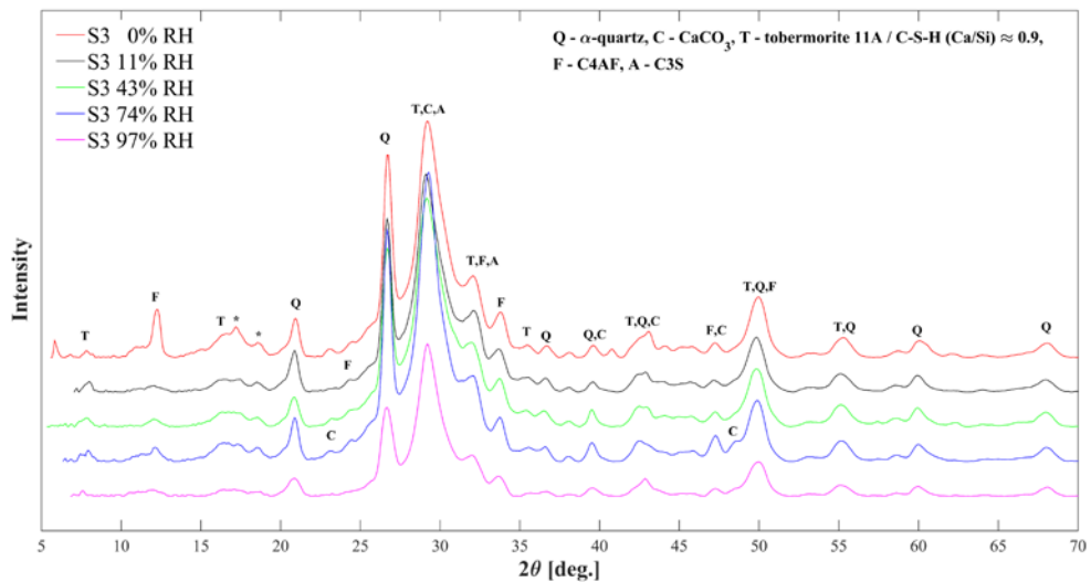
Figure SI2-2. Qualitative analysis of the X-ray ( \text{Cu } K\alpha_1=1.540598 \text{ \AA} ) powder diffraction results obtained on S3 hydrated cement paste with silica enrichment (C-S-H matrix with the approximate Ca/Si \approx 0.92 ) equilibrated at 0, 11, 43, 74 and 97% RH. To make the comparison with literature data easier, the diagrams, recorded with a molybdenum anode ( \lambda_{K\alpha_1} = 0.70932 \text{ \AA} ), were then calculated with respect to a copper anode ( \lambda_{K\alpha_1} = 1.540598 \text{ \AA} ). * - unidentified peaks in the proximity of 101 reflection of ordered 11Å tobermorite, also typical of nano-crystalline disordered tobermorite structure [5, 6], T – diffraction lines due to crystalline and semi-crystalline calcium silicate hydrates, 11Å tobermorite and C-S-H.
