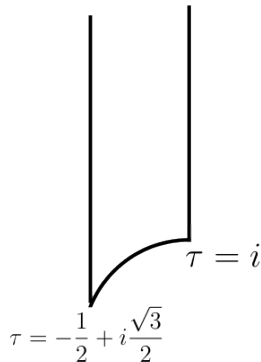
Figure 1: Fundamental domain for the modulus \tau .
