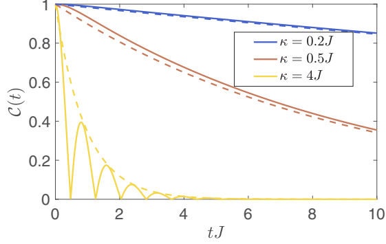
FIG. 3. Behavior of the coherence for the single impurity model. Here and in the following we compute Eq. (10) by numerical diagonalization of the corresponding reduced Lindbladian. Continuous lines are numerical simulation and dashed lines are an analytical approximation of Eqs. (16) and (17). Dissipation is fixed to \Gamma = 4J . The results for N = 4 are indistinguishable from those at N = 400 .
