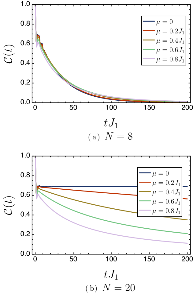
FIG. 12. The effect of noise on the coherence in the non-Hermitian SSH model with (a) N = 8 and (b) N = 20 , respectively. We take the W = 1 phase, where J_1 = 1 , J_2 = 1.8 , \Gamma = 0.5 , and the noise rate \mu is taken between 0 and 0.8J_1 . The final result is averaged over 1000 runs of randomly generated systems with the respective noise rates.
