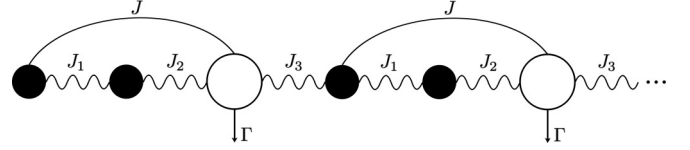
FIG. 8. Model (35) with a three-site unit cell.
