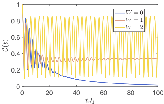
FIG. 10. Behavior of the coherence in the linear chain with three sites per cell, Eq. (35). We chose N = 8 , but the numerical results are not sensitive to N \bmod 3 . The winding number can assume values W = 0, 1, 2 . W also counts the number of edge modes localized near the first qubit. For W = 2 the dark-state manifold is a physical qubit and one sees Rabi oscillations in the coherence. Parameters are J_1 = 1 , \epsilon = 0 , \Gamma = 0.5 , J_2 = 0.3 , J = 0.7 , and J_3 fixes the value of W : J_3 = 0.2 ( W = 0 ), J_3 = 0.7 ( W = 1 ), and J_3 = 2 ( W = 2 ).
