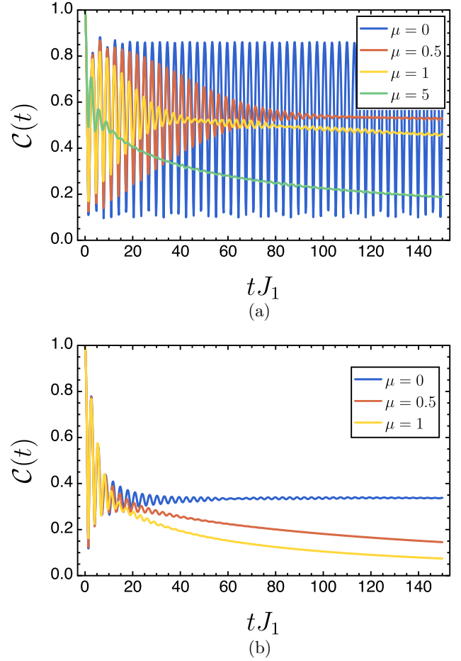
FIG. 13. The effect of noise on the coherence in the three-site unit-cell model with N = 8 . (a) Phase W = 2 with J_1 = 1 , J_2 = 0.3 , J_3 = 2 , J = 0.7 , and \Gamma = 0.5 . (b) Phase W = 1 with J_1 = 1 , J_2 = 0.3 , J_3 = 0.7 , J = 0.7 , and \Gamma = 0.5 . The noise rate \mu is taken to be 0, 0.5J_1 , and J_1 . The final result is averaged over 1000 runs of randomly generated systems with the respective noise rates.
