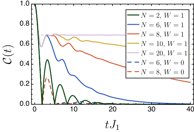
FIG. 7. Behavior of the coherence in the non-Hermitian SSH model with an even number of sites. Continuous lines are results in the topological phase ( W = 1 ) with parameters J_1 = 1 , J_2 = 1.8 , and \Gamma = 0.5 . Increasing N has the effect of exponentially increasing the (coherence) time scale \tau_{\text{coh}} at which the approximate dark state starts decaying. Dashed lines are for the topologically trivial phase ( W = 0 , J_1 = 1 , J_2 = 0.5 , \Gamma = 0.5 ). For N = 10, 20 the plot is indistinguishable from that of N = 8 . The thin dashed line is the asymptotic value given by Eq. (34). The intrinsic coherence lifetime of the qubit ( N = 2 ) is added for comparison. We observe that the lattice of cavities with W = 1 vastly improves the lifetime of the coherence.
