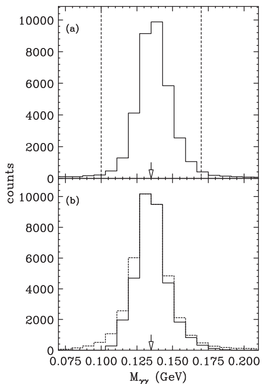
FIG. 1. Two-photon invariant mass distributions for (a) ep \rightarrow e\gamma\gamma p and (b) ep \rightarrow e\gamma\gamma(p) , with all relevant exclusivity cuts applied. The vertical dashed lines show the cuts used for ep \rightarrow e\gamma\gamma p . The solid (dashed) curve in the lower panel is with (without) the application of the \chi^2 cut discussed in the text.
