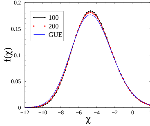
Figure 7. Distribution f(\chi) of the variable \chi introduced in (2.25), as measured on the TASEP with N = 100 and N = 200 . Blue curve: limiting distribution predicted by the ansatz (2.26).
