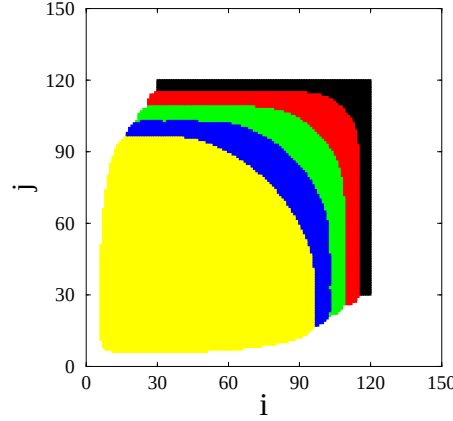
Figure 9. Average shape of a droplet of size N = 90 embedded in a system of size N_{\text{sea}} = 150 for T/T_c = 0.5 , at times \alpha t multiples of 20.
