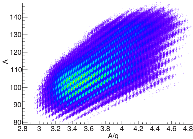
FIG. 2. Mass versus mass-to-charge ratio obtained from the magnetic rigidity of the ions and their time of flight through VAMOS++. The diagonal bands of loci correspond to a unique charge state.
