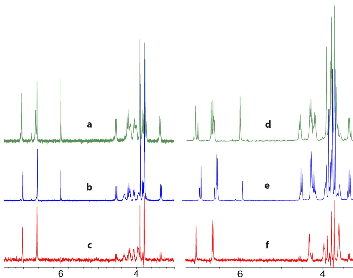
S8 : ^1\text{H} NMR spectra of compound 9a (left) and 9s (right) for the degassed solutions (spectra a and d) ; in presence of xenon (spectra b and e). ^{129}\text{Xe} - ^1\text{H} SPINOE spectra of compounds 9a (spectrum c) and 9s (spectrum f).
