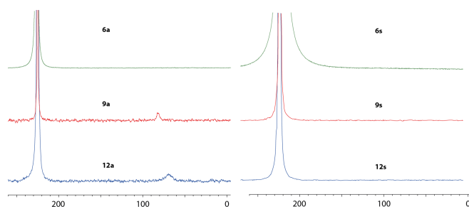
Figure 2. One-scan ^{129}\text{Xe} NMR spectra of the samples of 6 ( a and s ), 9 ( a and s ), 12 ( a and s ). The subscripts a and s refer to anti and syn arrangement of the linkers. Spectra have been recorded at 11.74 T and 293 K. Each sample contained 0.3 \pm 0.03 mg of cryptophane (0.4 - 0.5 mM) in 600 \mu\text{L} of 1,1,2,2-tetrachloroethane- d_2 and ca. 10 mg of xenon (representing a concentration of ca. 100 mM).
