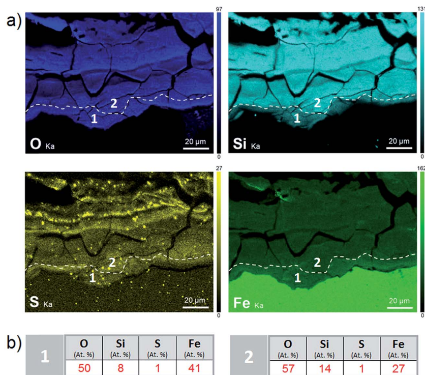
Fig. 9 (a) EDS maps of the metal/corrosion product interface on a cross-section of the Batx sample, where O ( K\alpha ) is presented in blue, Si ( K\alpha ) in light blue, S ( K\alpha ) in yellow and Fe ( K\alpha ) in green, and (b) average quantification of EDS point analyses performed at two points on the metal/corrosion product interface.
